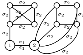
Figure 26: Either a cycle with constant weight is complete or all its vertices are linked to one end-vertex of e_1 .
