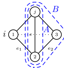
Figure 5: Cycle C with w(e) < w_1 = w_2 .
