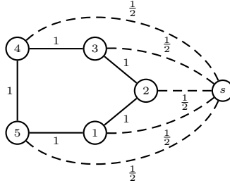
Figure 3: Weighted graph G' built from G .
