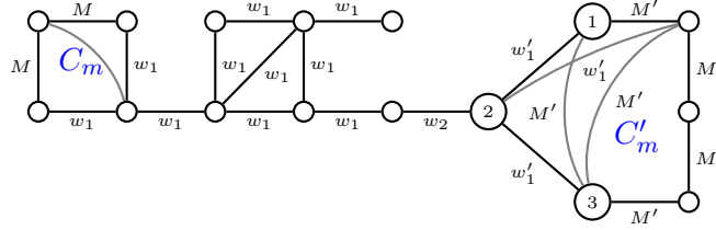
Figure 22: |E_1| \geq 2 , \sigma(N) = w_1 < M , and w_1 \leq w_2 < w'_1 = w'_2 < M' .
