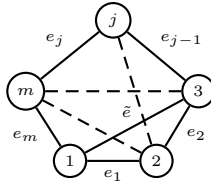
Figure 19: \{1, j\} \notin E(C) with j \geq 4 .
