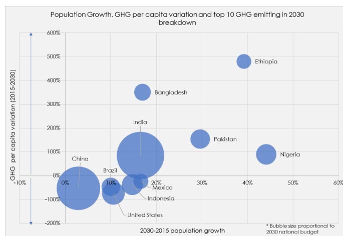
Figure 9: Emissions and population change for the top 10 countries
