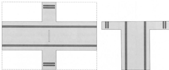
Figure 3. Tunic with long sleeves, woven to shape, in one piece. Drawing: Mahmoud Bakhit © Ifao, after Carroll 1988, fig. 12 A.
