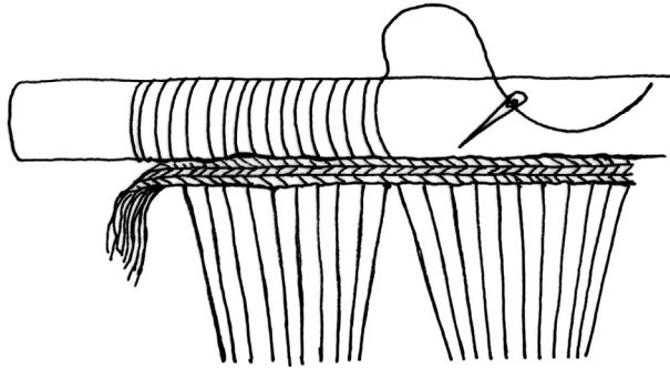
Fig. 3. Diagram of the meeting and reversal of weft yarns in tapestry weave. After Seagroatt (1979), 14.
