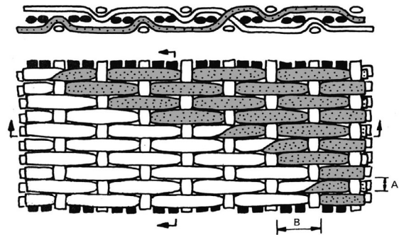
Fig. 4. Diagram of the structure of taqueté . Drawing by courtesy of D. De Jonghe.
