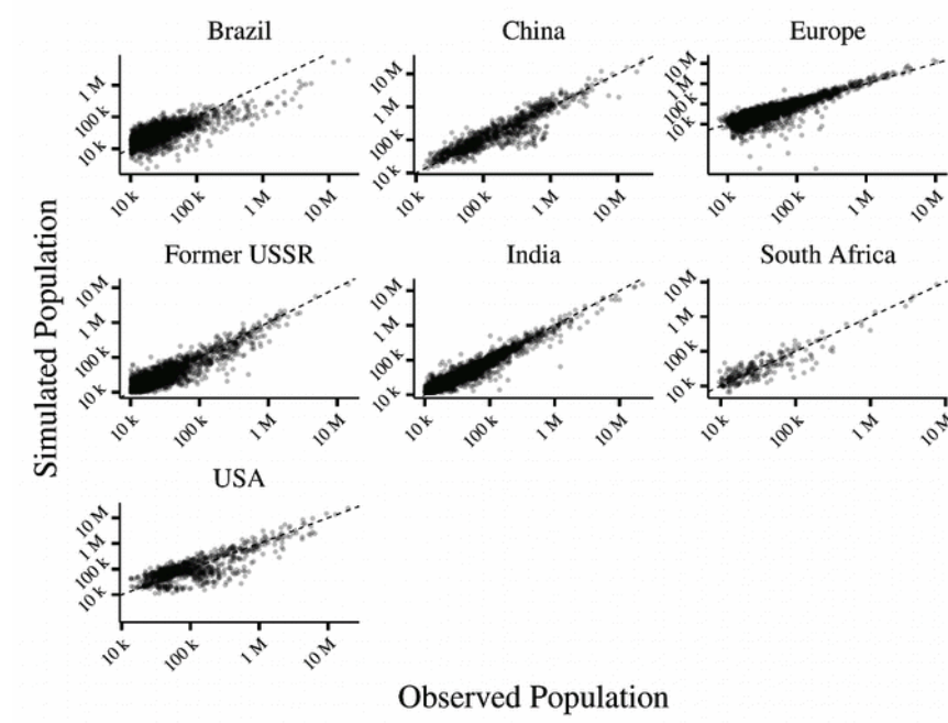
Figure 6 Comparing observed final city size and simulated with Gibrat's model
