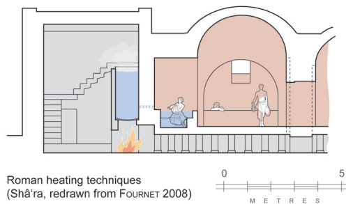
Fig. 2 – From Roman Baths to Hammam: Evolution of Heating Techniques (Th. Fournet, after FOURNET 2008a and CHARPENTIER 1995)
