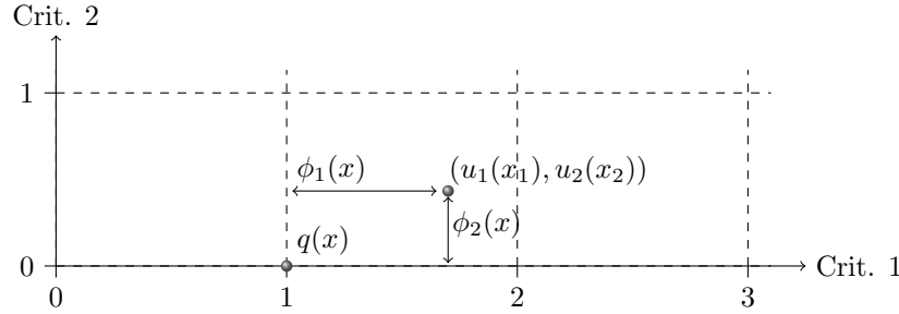
Figure 5: Illustration of q(x) , \phi_1(x) and \phi_2(x) .
