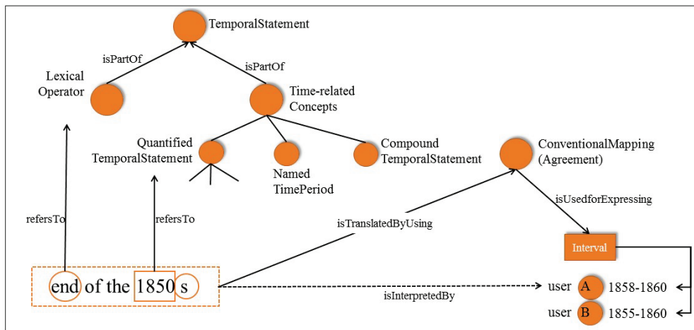
FIG. 1 – Components of a TemporalStatement and their interrelations.
