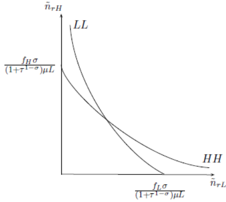
Figure 3: HH and LL in the (\tilde{n}_{rH}, \tilde{n}_{rL}) plane
