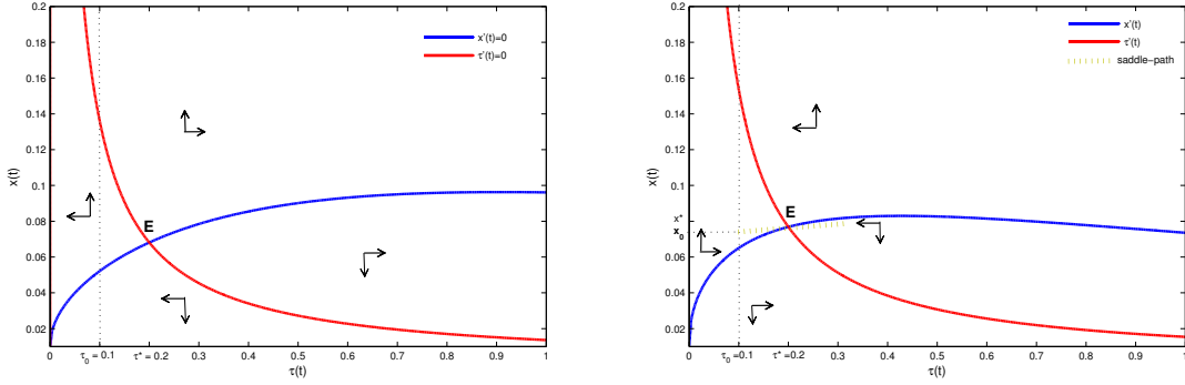
Figure 2: Phase Diagrams when \phi > 0 (left) and \phi < 0 (right) and \gamma = \hat{\gamma}^1
