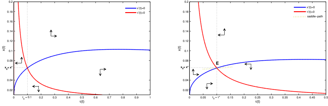
Figure 1: Phase Diagrams when \phi > 0 (left) and \phi < 0 (right) and \gamma = \hat{\gamma}^0
