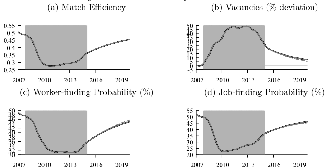
Figure 6: Match Efficiency: The Labor Market
