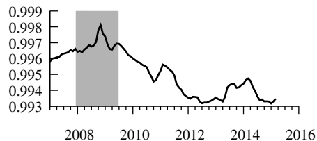
Figure 3: The Financial Shock
