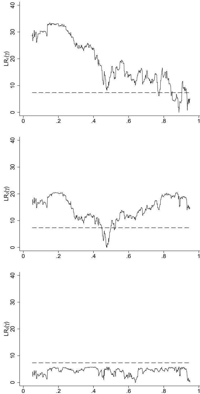
Figure 3: Likelihood Ratio test and confidence interval construction for the three thresholds tested. Vertical axis: LR-test; horizontal axis: percentiles of the threshold variable K_{R/F} . The dashed horizontal line represents the 5% critical value of the test.
