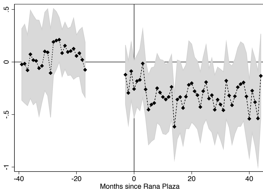
Figure 5: Monthly triple difference estimates Time=0 for April 2013. The point estimates are reported in Table A-4 in the Appendix.
