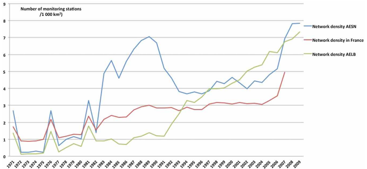
Fig. 3. Changes in monitoring networks' density (number of monitoring stations/1,000 km 2 ) in France, Seine-Normandie (AESN) and Loire-Bretagne (AELB) water agencies from 1971 to 2009 (Chemlal & Meybeck, 2015).
