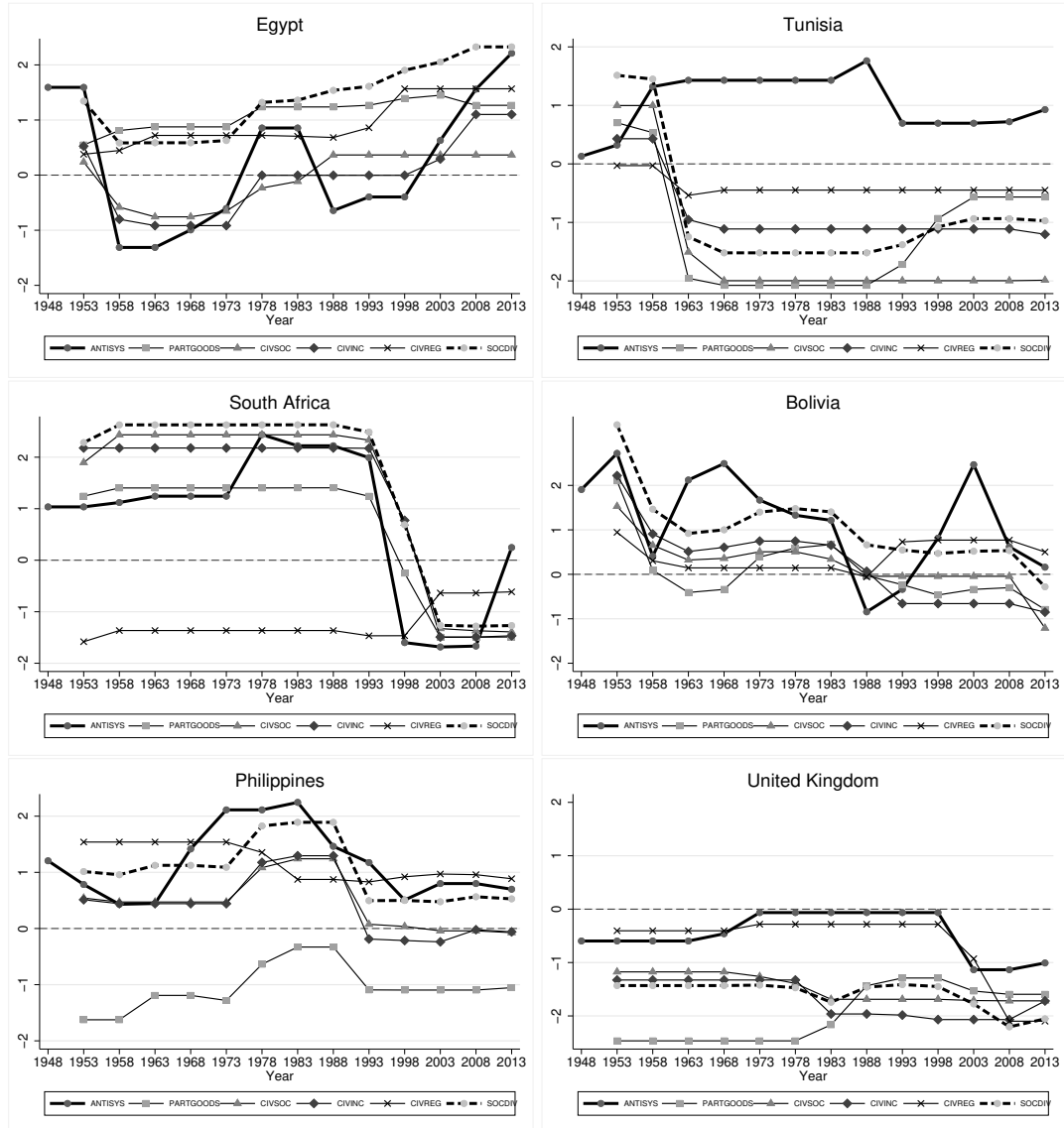
Figure 7: ANTISYS and SOCDIV components, selected countries
