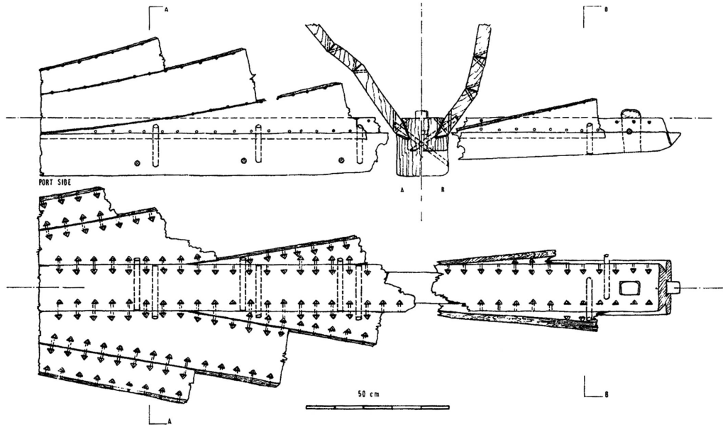
Figure 22. Giglio shipwreck: reconstruction of keel and planking (drawing S. Dobbs, from Linder and Kahanov, 2003).
