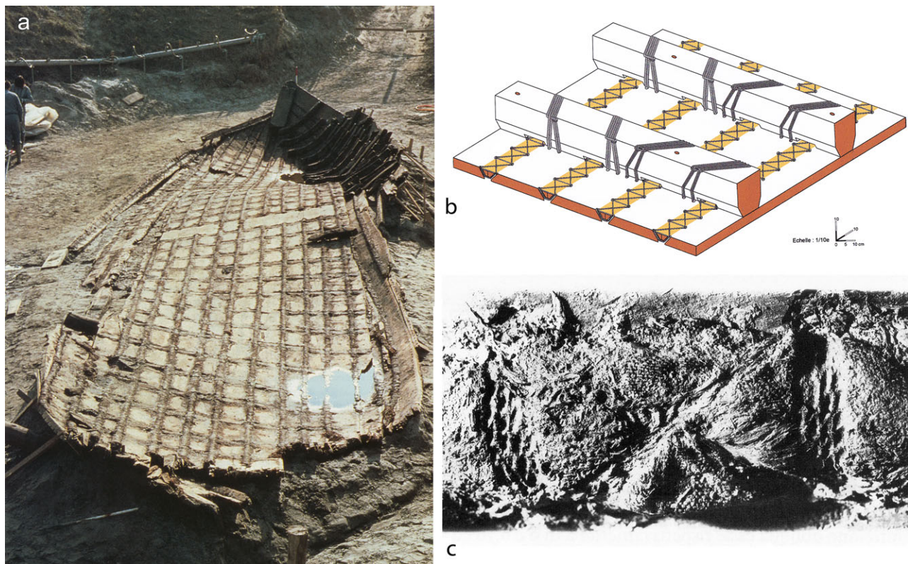
Figure 7. Comacchio shipwreck: a) general view of the hull after dismantling the frames for recovery, with the stem visible at the far end (from Berti, 1990: 25); b) axonometric illustration of the sewing systems (drawing S. Marlier; Marlier, 2005: fig. 135a); c) detail view of the sewing system (from Berti, 1990: 30, fig. 4).
