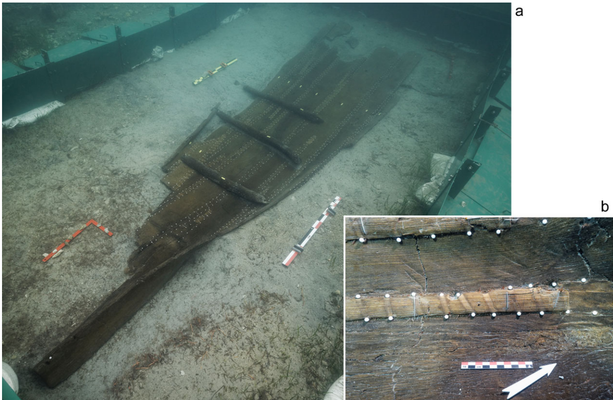
Figure 3. Zambratija shipwreck: a) general view of the hull during the 2013 excavation (photo Ph. Groscaux, AMU, CNRS, CCJ); b) detail view of the sewing pattern (photo Ph. Groscaux, AMU, CNRS, CCJ).
