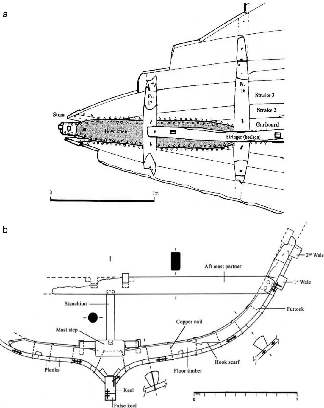
Figure 32. Ma'agan Mikhael shipwreck: top view of the sewing on the bow knee; transversal main section of the hull (from Linder and Kahanov, 2003).
