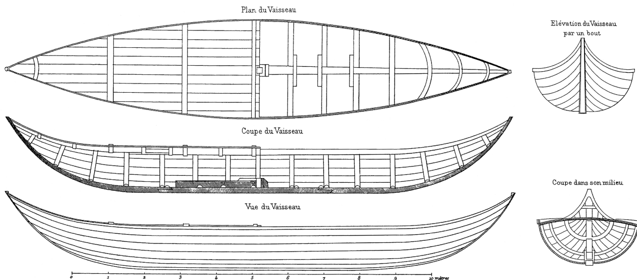
Figure 16. Golo shipwreck: plan, sections and elevations (from Pâris, 1892).
