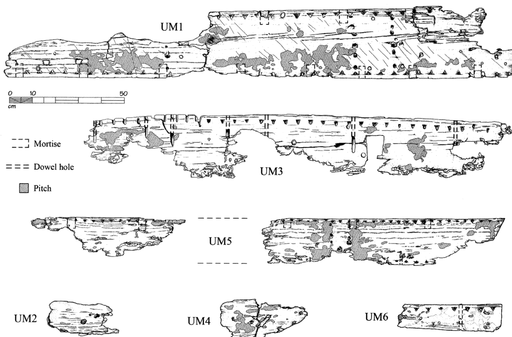
Figure 24. Pabuç Burnu shipwreck: planks remains (from Polzer, 2010).
