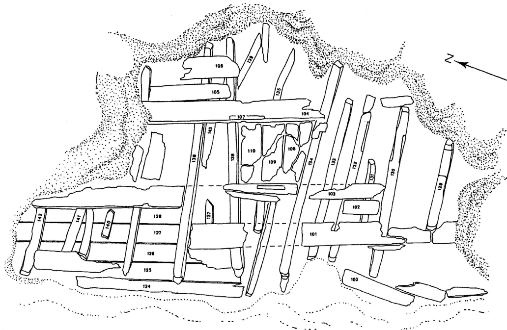
Figure 38. Plane 1: general plan in the centre part. Note the disturbance of the frames in the axial part due to the ripping out of the keel (drawing M. Rival, from Pomey, 2002b).
