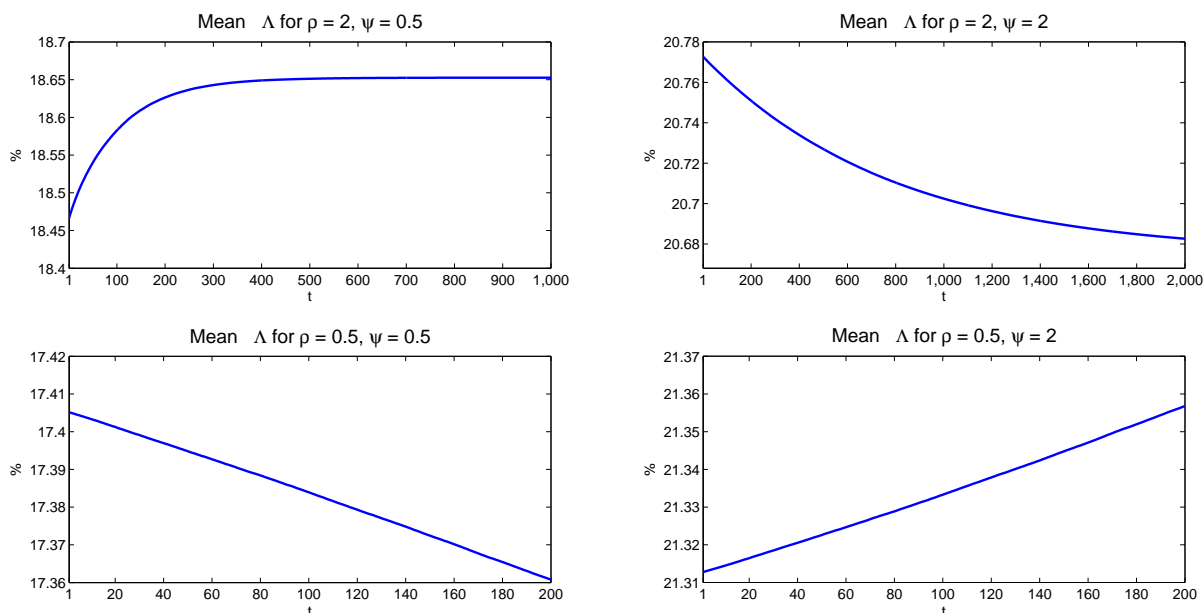
Figure 8: Evolution of the mean government share over time. The two graphs on the top consider the case of \rho = 2 . The two graphs on the bottom consider the case of \rho = 0.5 . Graphs on the left correspond to the substitutes case ( \psi = 0.5 ) and graphs on the right to the complements case, ( \psi = 2 ). When \rho = 2 we have convergence to the balanced-budget government share that is either below (substitutes) or above (complements) the first-best government share of 20%.
