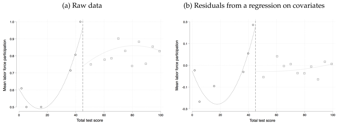
Figure 2: Reduced form graph
