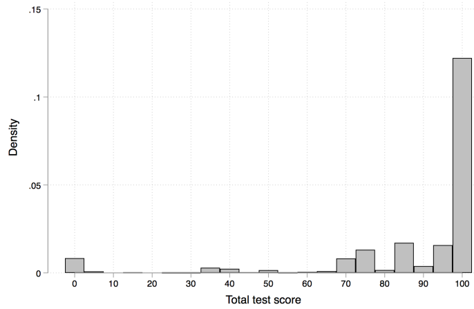
Density plot over the whole sample
