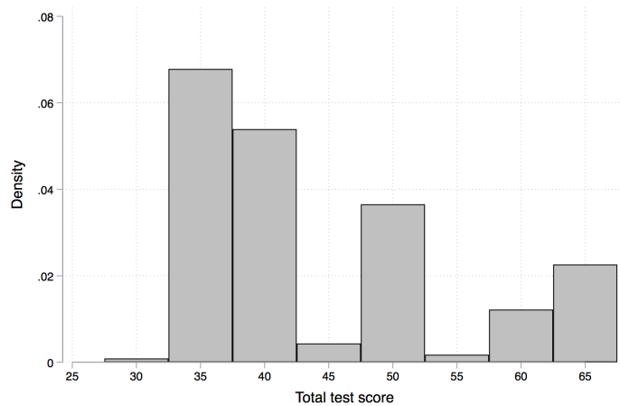
Density plot zoomed on the threshold
