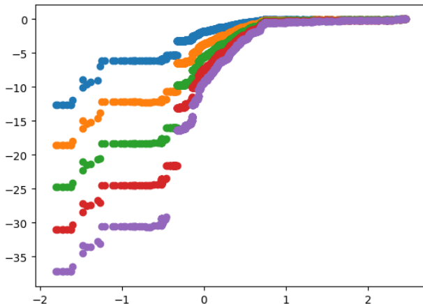
Fig. 5 Measures of \mu_i(q, \epsilon) in a double logarithmic projection ( x axis is the metric which is the line impedance, y axis is q moment of the measures)
