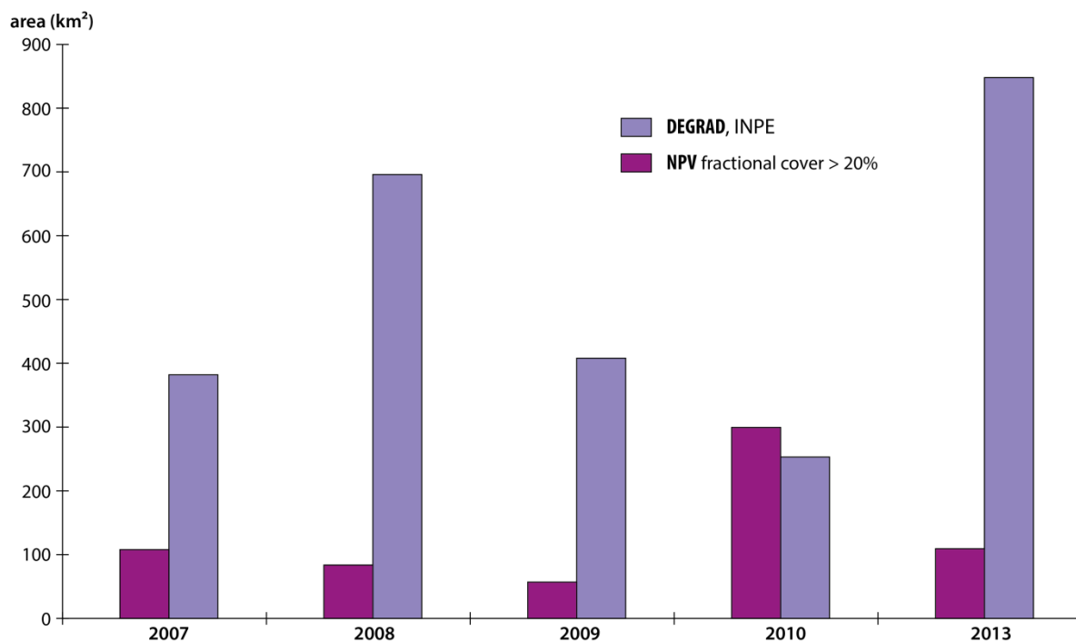
Figure 11: Assessment of forest degradation area in Paragominas municipality estimated using the DEGRAD – INPE method ( www.obt.inpe.br/OBT/assuntos/programas/amazonia/degrad ) and from the CLASlite method (this study); only pixels with the highest values of NPV fractional cover (>20%) were selected.
