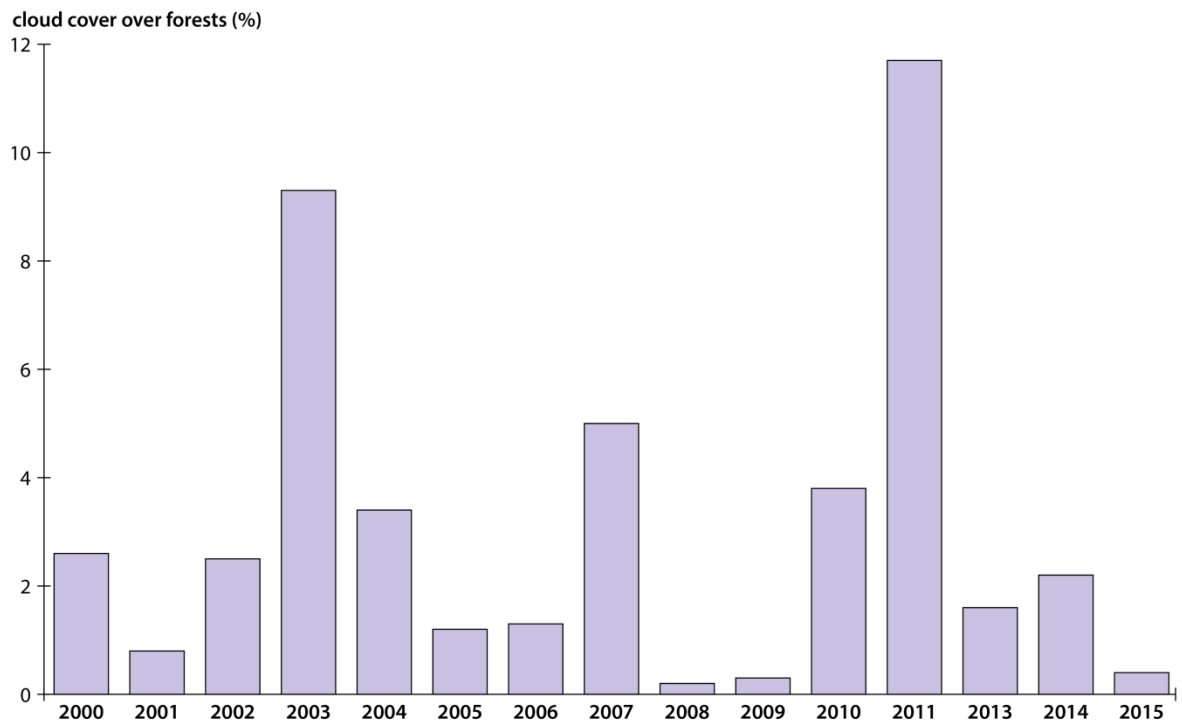
Figure 3: Remaining cloud cover over the forested area in Paragominas municipality
