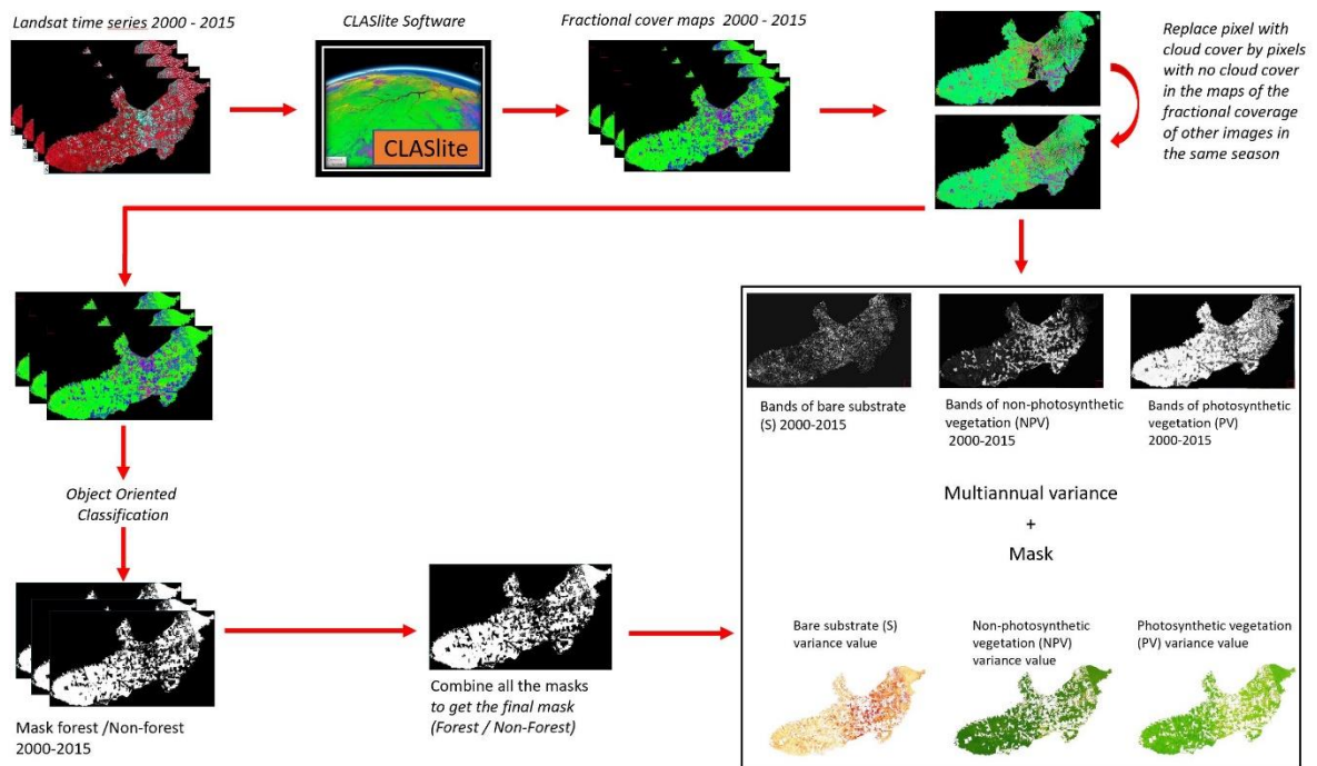
Figure 2: CLASlite software processing of Landsat images for the assessment of photosynthetic vegetation (PV), non-photosynthetic vegetation (NPV), bare substrate (S) bands in a multiannual period, and non-forest mask building from CLASlite results.
