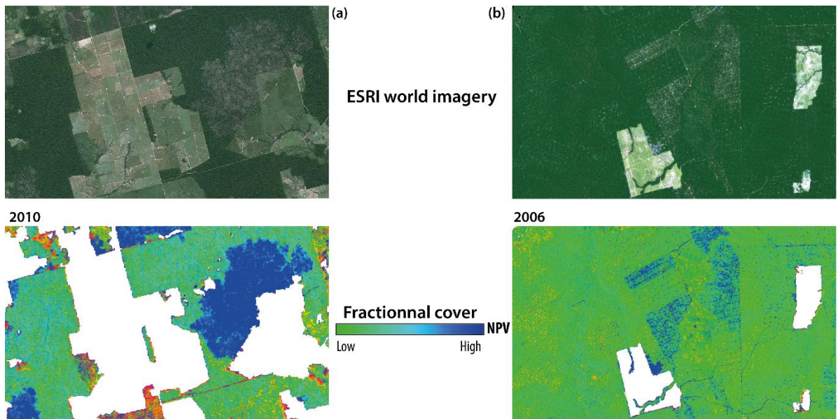
Figure 10: Forest degradation patterns in Paragominas observed via NPV fractional cover; (a) Zonal disturbance (fuel wood gathering) with homogeneous distribution of non-photosynthetic vegetation in the degraded area and (b) selective logging, with roads and regularly shaped gaps in the plots visible in the NPV fractional cover map.
