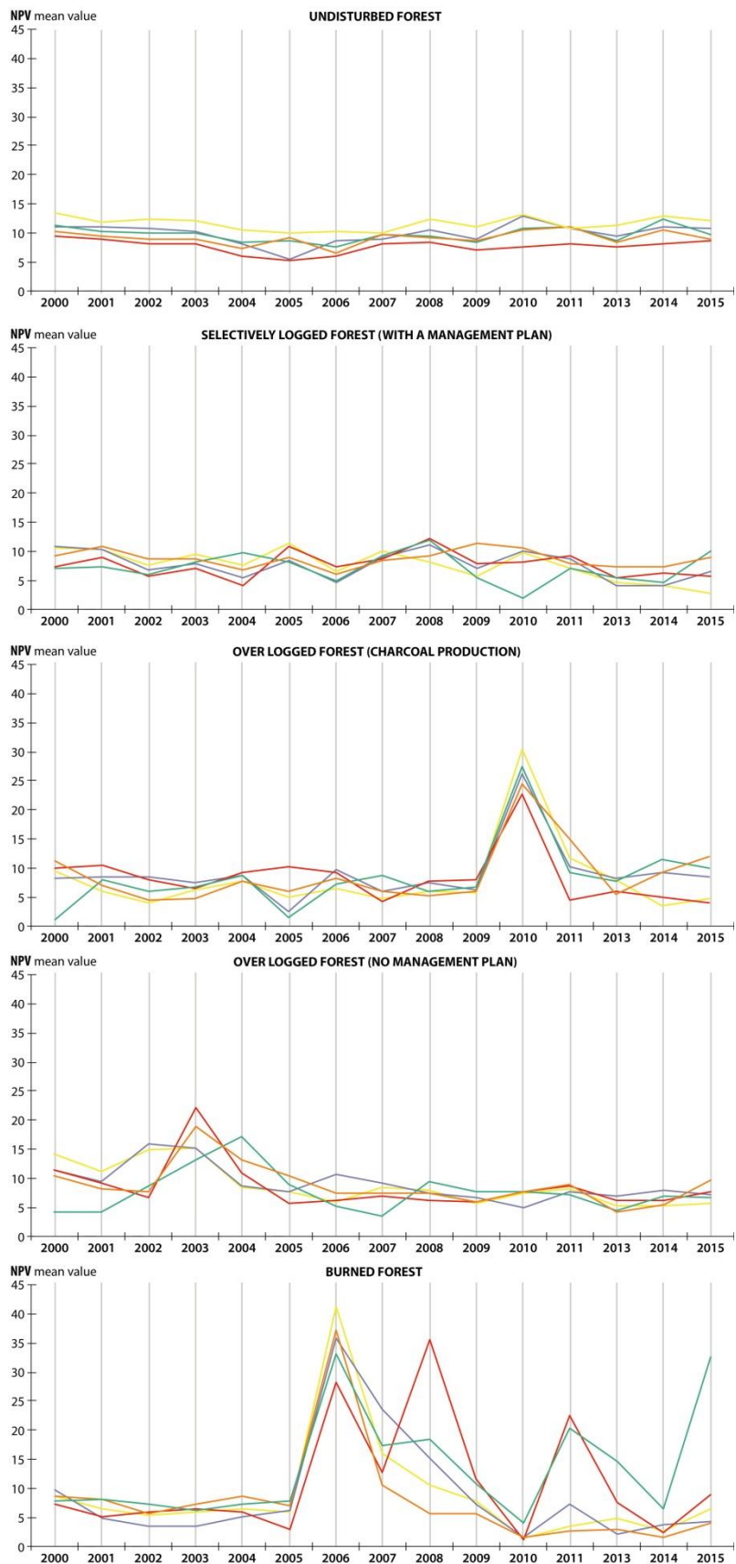
Figure 6: NPV mean values for the 5 reference plots of undisturbed forest and each of the four degradation types.
