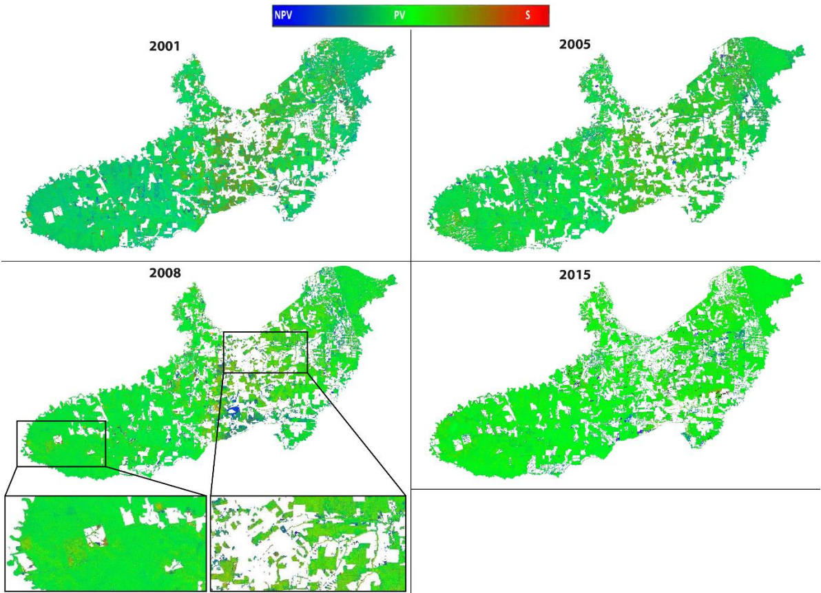
Figure 4: Four annual fractional cover maps (2001, 2005, 2008 and 2015) processed with CLASlite software using Landsat images. With a zoom on two zones in the 2008 fractional cover map.
