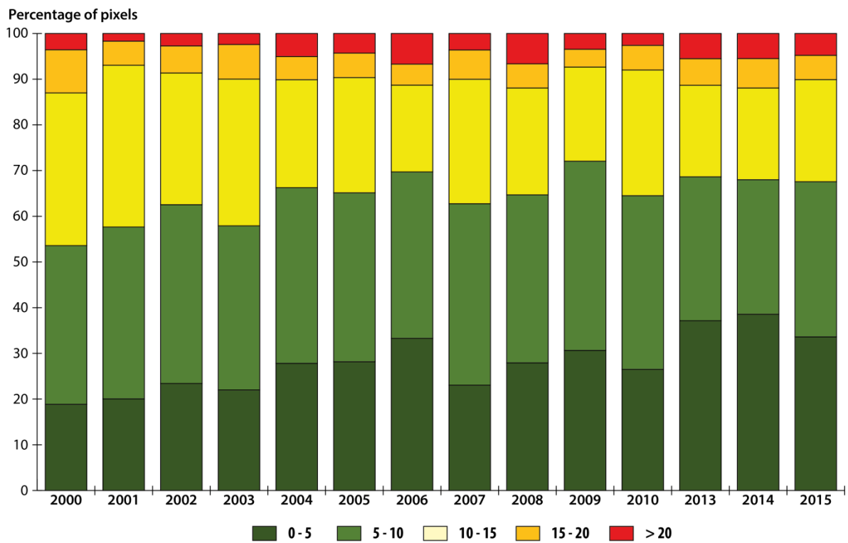
Figure 9: Percentage of pixels in five classes of NPV fractional cover value on the forested area of the municipality of Paragominas; distribution is displayed for each year over the period 2000-2015.
