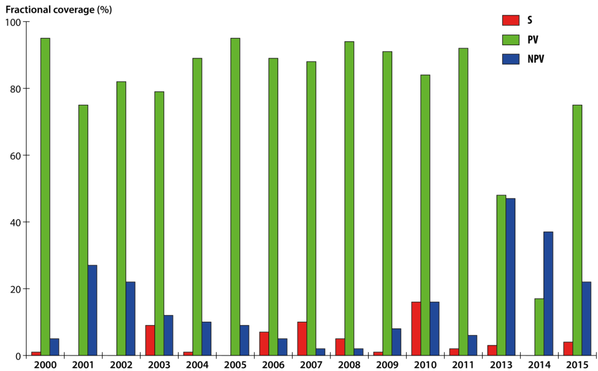
Figure 5: Fractional cover (in %) of bare Substrate (S), Photosynthetic Vegetation (PV) and Non-photosynthetic vegetation (NPV) during the period 2000-2015 for a 3x3 pixel window; the pixel at the center of the window was affected by a logging gap in 2001 and 2013.
