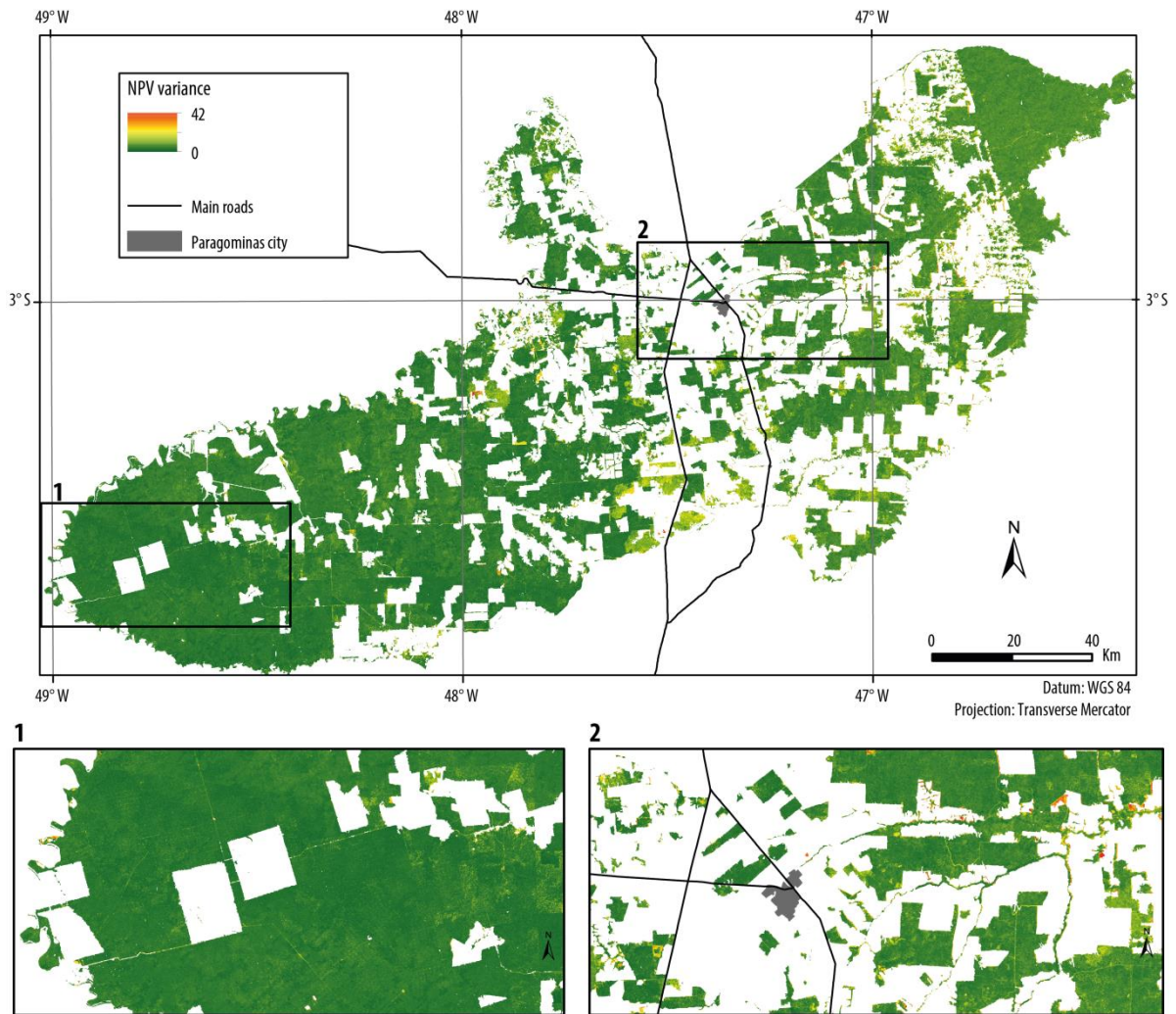
Figure 8: Mapping of the Non-Photosynthetic Vegetation (NPV) variance calculated over the period 2000-2015 in the municipality of Paragominas, with a zoom on two zones.
