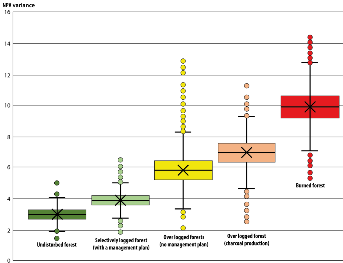
Figure 7: NPV variance calculated for undisturbed forest and each of the four degradation types; the box-plots report the median value and the distribution of variances computed for each pixel of the reference plots over the period 2000-2015.
