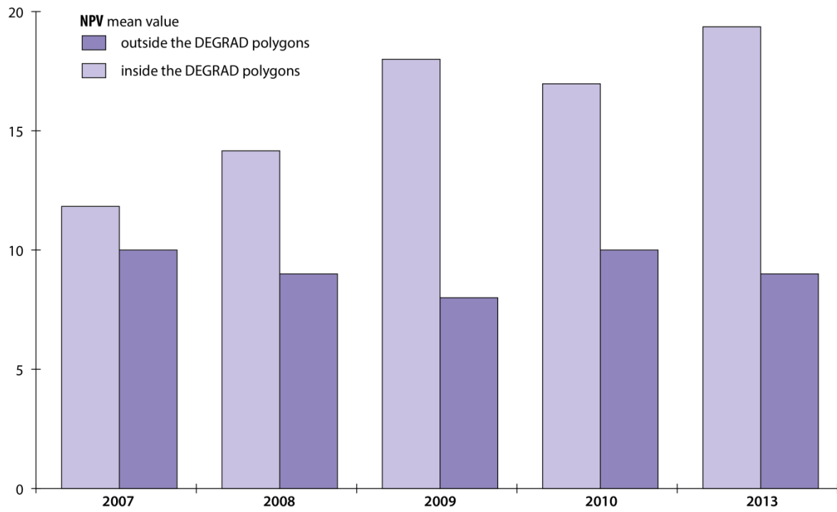
Figure 12: NPV mean value calculated for all the pixels inside and outside the polygons recorded by DEGRAD – INPE mapping.
