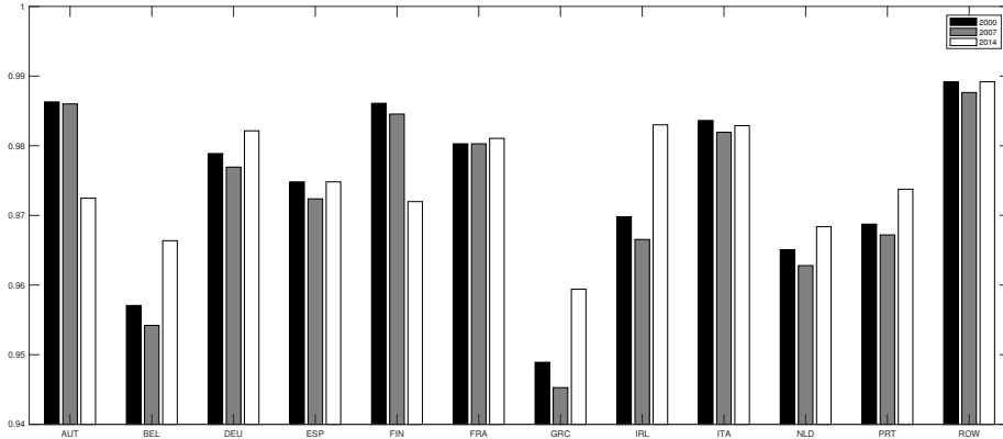
Figure A-3: Average country centrality based on indegree.
