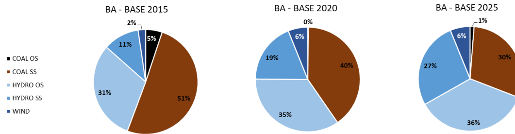
Figure 3. Baseline Scenario projections of electricity generation in Bosnia and Herzegovina for the years 2015, 2020 and 2025. The denominations OS and SS used for some technologies, respectively, mean "Outside Sava River basin" (OS) and "In Sava River basin" (SS) (source: Energy Strategy for BiH until 2035)
