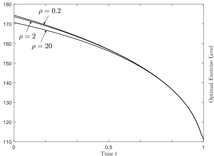
Fig. 3. The early exercise boundaries of a down-and-out step call option for different values of \rho . Parameters values: K = 100 , H = 95 , r = 0.05 , \delta = 0.035 , \sigma = 0.3 , n = 300 , tol = 0.0001 , T = 1 .
