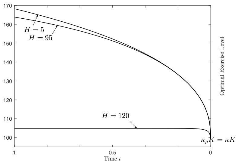
Fig. 4. The early exercise boundaries of a down-and-out step call option for different values of H . Parameters values: K = 100 , \rho = 20 , r = 0.05 , \delta = 0.05 , \sigma = 0.3 , n = 300 , tol = 0.0001 , T = 1 .
