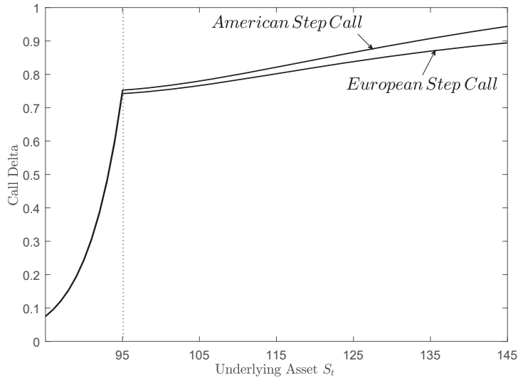
Fig. 5. The delta hedging ratio ( \partial SC/\partial S ) for a down-and-out step call option. Parameters values: K = 100 , H = 95 , \rho = 20 , r = 0.05 , \delta = 0.05 , \sigma = 0.3 , n = 300 , tol = 0.0001 , T = 1 .
