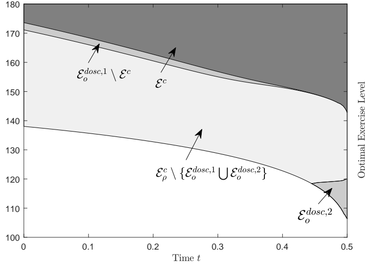
Fig. 2. Optimal exercise regions \mathcal{E}^c \subseteq \mathcal{E}_o^{dosc} \subseteq \mathcal{E}_\rho^c . \mathcal{E}^c is the exercise region of a vanilla call option in the market \mathcal{M}(r, \delta) . \mathcal{E}_o^{dosc} = \mathcal{E}_o^{dosc,1} \cup \mathcal{E}_o^{dosc,2} is the exercise region of a down-and-out step call option in the configuration \kappa K \geq H \geq \kappa_\rho K > K . \mathcal{E}_\rho^c is the exercise region of a vanilla call in the market \mathcal{M}(r + \rho, \delta + \rho) . Parameters values: K = 100 , H = 120 , \rho = 0.2 , r = 0.05 , \delta = 0.035 , \sigma = 0.3 , n = 300 , tol = 0.0001 , T = 0.5 .
