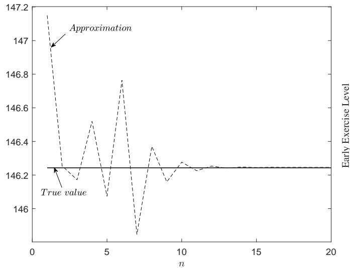
Fig. 6. Approximation vs. “True value” of the EEB of a down-and-out step call option at the point t = 0 . Parameters values: K = 100 , H = 95 , \rho = 26.34 , r = 0.05 , \delta = 0.07 , \sigma = 0.3 , n = 300 , tol = 0.0001 , T = 1 .
