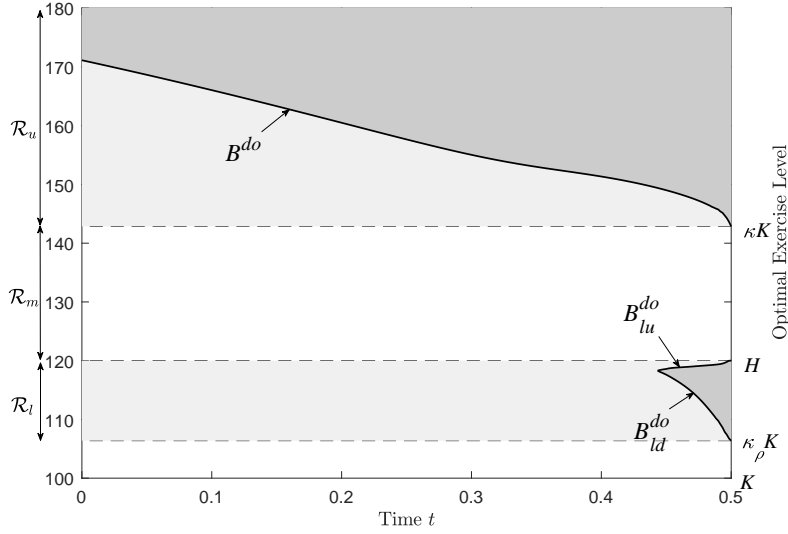
Fig. 1. The early exercise boundaries of a down-and-out step call option in the configuration \kappa K \geq H \geq \kappa_\rho K > K . Parameters values: K = 100 , H = 120 , \rho = 0.2 , r = 0.05 , \delta = 0.035 , \sigma = 0.3 , n = 300 , tol = 0.0001 , T = 0.5 .
