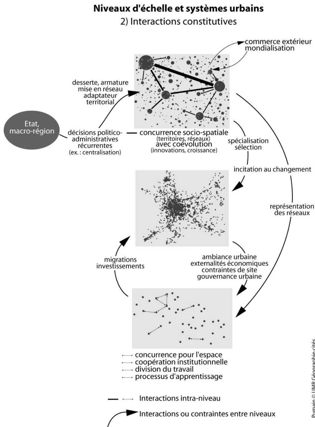
Figure 2 : Interactions constitutives
