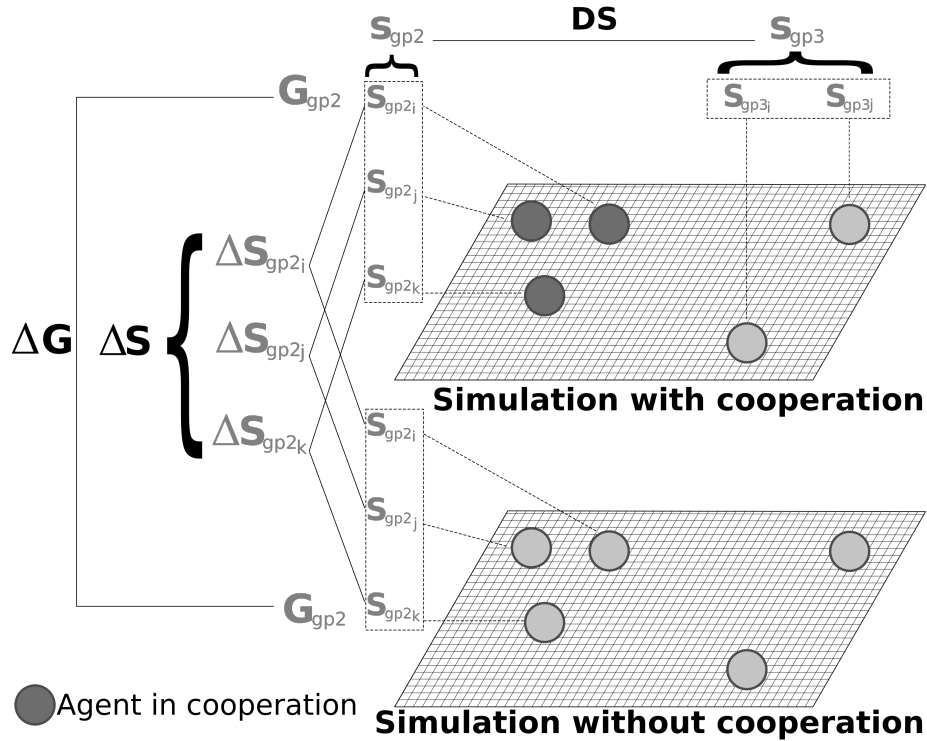
Figure 2: Explanation of the three indicators used to summarize the outcomes of simulations: \Delta S , DS and \Delta G . The dashed lines indicate the attributes of agents ( S = size). The G measures the Gini index of sizes within a group of agents. The continuous lines indicate computations of difference. The curly braces indicate computations of average.
