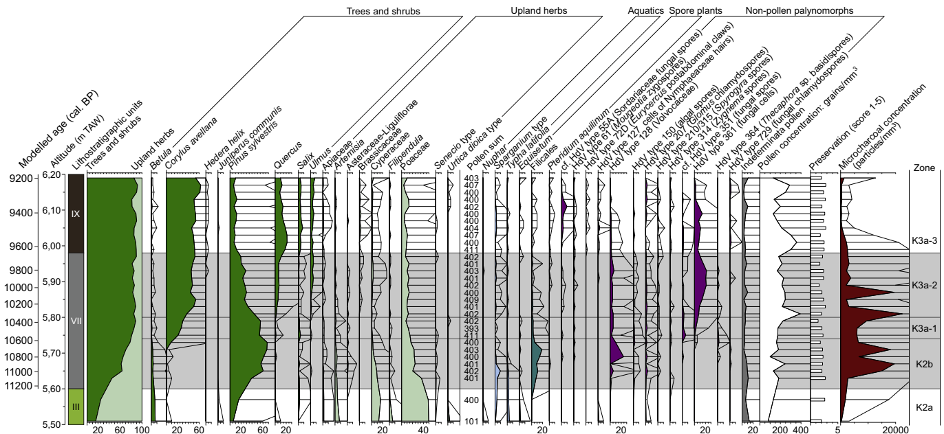
Fig. 5. Pollen percentage diagram (selected taxa) of the analysed sequence in T3. Full counts in supplementary data Table 2. Ages have been modelled according to the age-depth model of Blaauw (2010), based on the selected dates of the Bayesian analysis.
