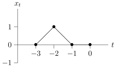
Figure 5: The resource stream x^5 = (0, 1, 0, 0) .
