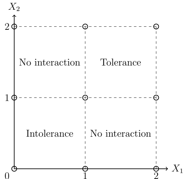
Figure 1: Decision strategies.
