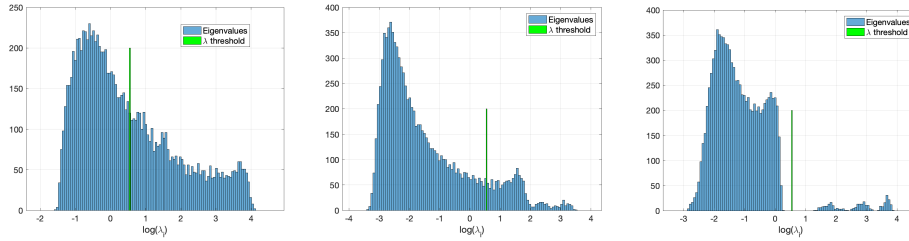
Fig. 1 Distributions of the logarithm of the eigenvalues of three covariance matrix estimates. Left side: Eigenvalues (log) of the SCM of the observations; Middle: Eigenvalues (log) of the Tyler covariance matrix of the observations; Right side: Eigenvalues (log) of the Tyler covariance matrix of the whitened observations. Observations contain K = 3 sources embedded in a multivariate K-distributed noise with shape parameter \nu = 0.5 , and a Toeplitz coefficient \rho = 0.8 . m = 100 , N = 1000 ( c = 0.1 ), and the (log) Marčenko-Pastur upper bound is here: \log(\bar{\lambda}) = \log(1.7325) .
