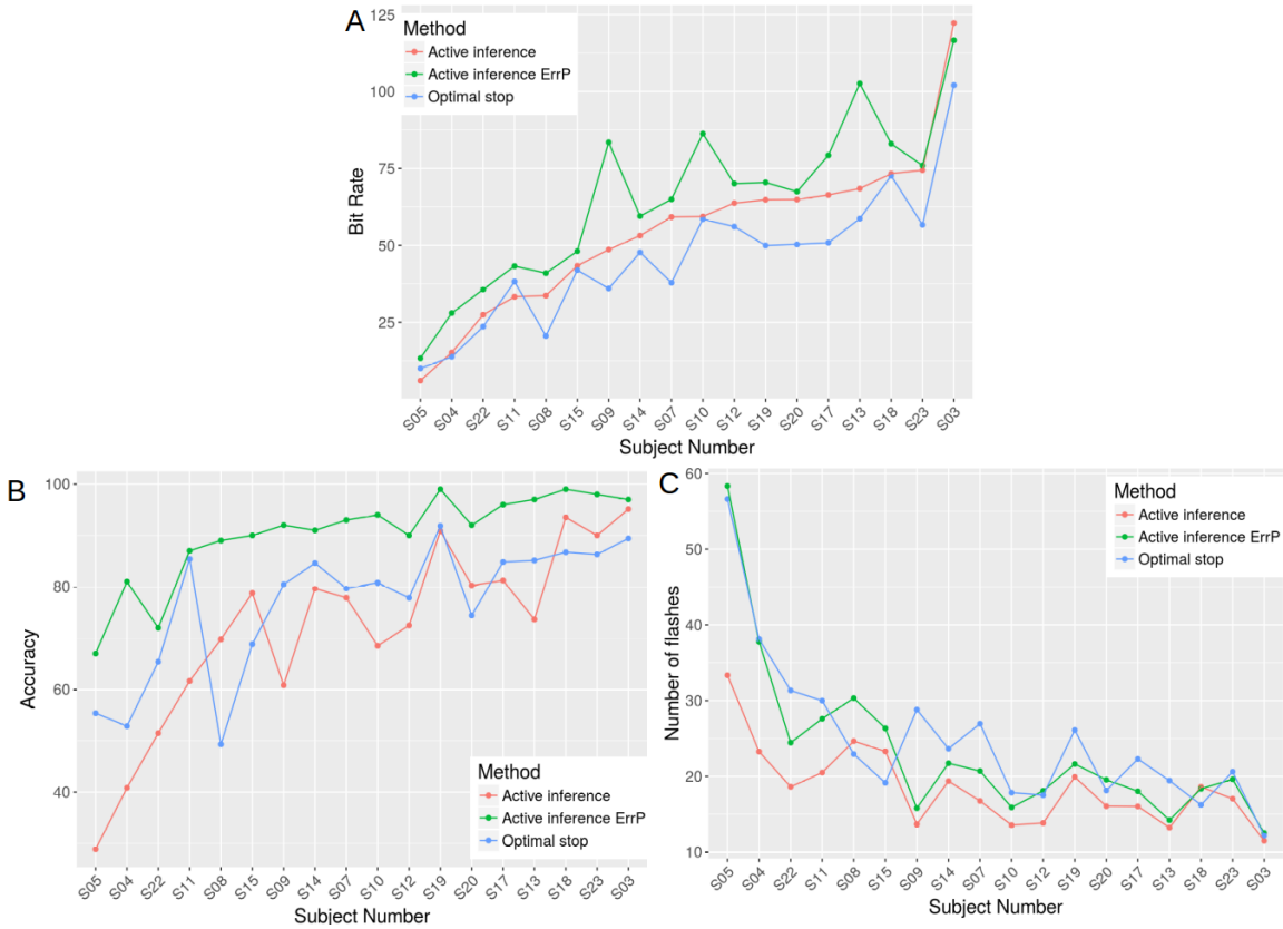
Figure 10: Comparison of (A.) Bit Rate, (B.) Accuracy and (C.) Mean number flashes, of Active inference basic (in red), AI with realistic ErrP classifier (in green) and Optimal stopping (in blue) across subjects (sorted by bit rate from left to right).
