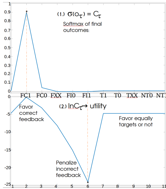
Figure 4: Upper figure: Softmax function yielding output values between 0 and 1 ( y-axis ) for each observation within the set \mathbb{O} ; from FC1, FC0, FXX, FIO, FI1 which refer to feedback observations ( o^{(2)}, o^{(3)}, \dots, o^{(6)} ) and T1, T0, TXX, NT0 and NT1 denoting target/non-target observations o^{(7)}, o^{(8)}, \dots, o^{(11)} ( x-axis ). Bottom figure: Logarithm of the softmax encodes a utility function, in which we favour the correctly spelled letter – FC1, and penalize feedback incorrect FI1 and FIO, and undefined FXX feedback; while equally favouring the apparition of target T, non target NT or undefined TXX observations.
