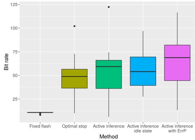
Figure 9: Comparison in bit rate (bit/min) between fixed flash, optimal stopping 0.9, AI basic, AI of lookAway, and AI + realistic ErrP. All methods significantly differ from one another ( p < 0.01 ).
