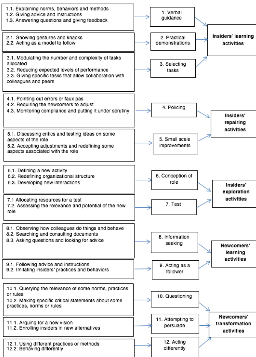
Figure 1 - Data structure
