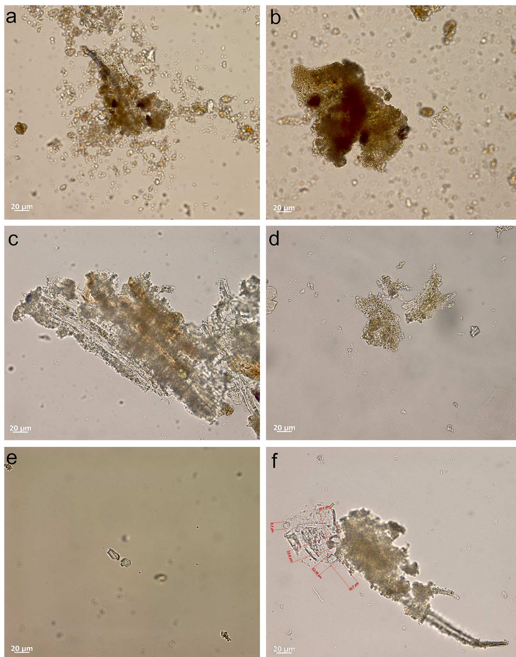
Fig 27. Examples of Podocarpus residues and comparative plant material. a and b) cf. Podocarpus sp. tissue recovered from the medial and proximal surfaces of 1136; c–f) an example of a polygonal starch granule from the proximal surface of 1170 (c) in comparison to articulated fibres (d), granular tissue (e) and starch granules (f) from Podocarpus falcatius stem reference material (x400, transmitted light).
