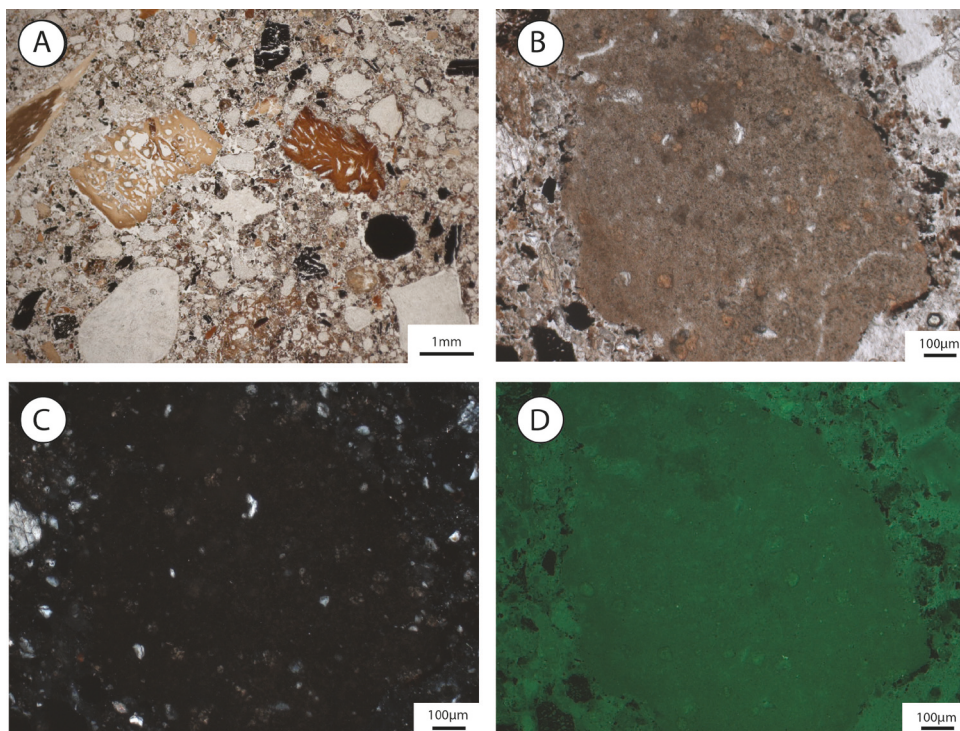
Fig. 21. Microphotographs of EBC-12-08. 21A) Bone fragments are relatively common here, but still exhibit evidence of dissolution. PPL. 21B) A nodule of hydroxylapatite that has been heated, based on measurements collected with the microFTIR directly on the thin section. PPL. 21C) Same view, but XPL. 21D) Same view, but under blue light fluorescence.
