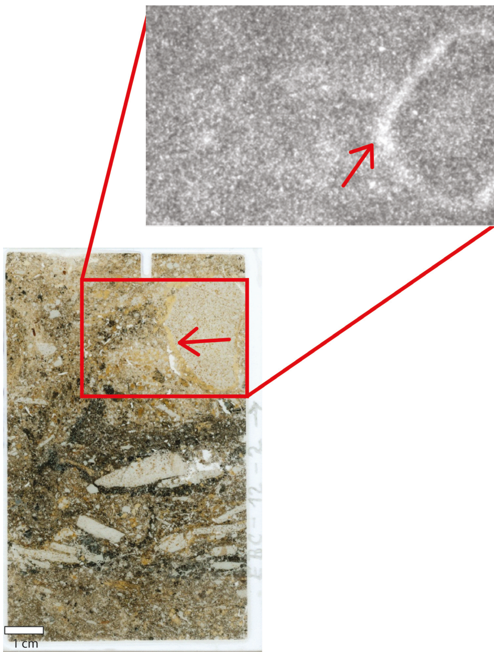
Fig. 13. Autoradiography image of a portion of sample EBC-12-02. The white ring (indicated by the arrow) is the taranakite crust forming on the quartzite block. The slight variation in morphology compared to the thin section is because the image was produced from the chip. These results indicated that the taranakite is the potassium-rich end member, an observation confirmed by the SEM-EDS results.
