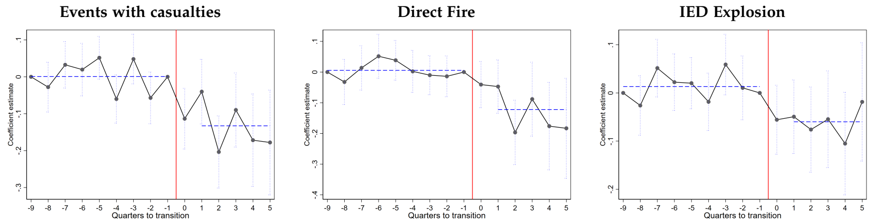
Figure 6: Event Studies around the Security Transfer to ANSF (SIGACTs)
