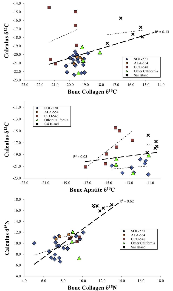
Fig. 3. Comparison of \delta^{13}\text{C} in bone collagen (top) and apatite (middle) and \delta^{15}\text{N} from bone collagen (bottom) against isotopes from calculus, by individual.
