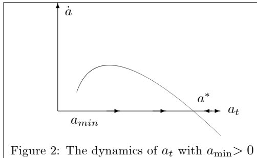
Figure 2: The dynamics of a_t with a_{\min} > 0
