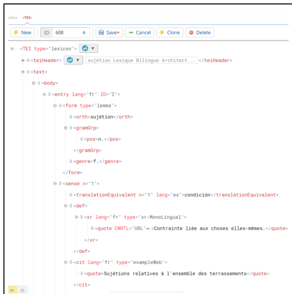
Figure 4. Recreating TEI-LMF serialization of an entry directly in Lexonomy
