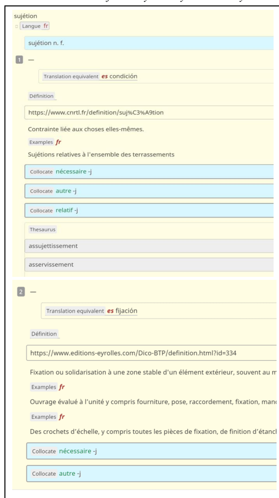
Figure 5. Style sheet of an entry defined directly in Lexonomy
