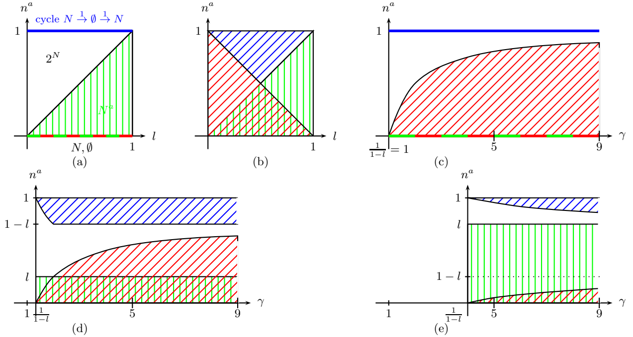
Fig. 2. Phase diagram for Situation 1: (a) \gamma has minimum value \frac{1}{1-l} ( r = 0 ); (b) \gamma \rightarrow \infty ; (c) l = 0 ; (d) l \in [0, 1/2] ; (e) l \in [1/2, 1] . Color code: white= 2^N , blue=cycle, red= N^c , green= N^a
