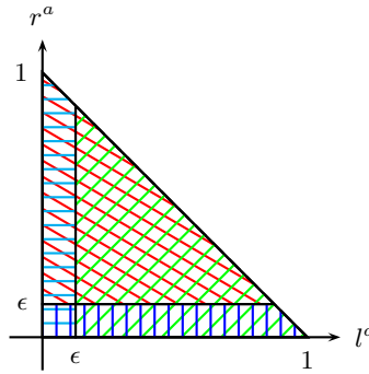
Fig. 4. Phase diagram for Situation 3, with l^c, r^c > \epsilon . Color code: green= N^a , red= N^c , cyan=almost consensus ‘no’ ((3) or (11)), blue=almost consensus ‘yes’ (4) or (12)
