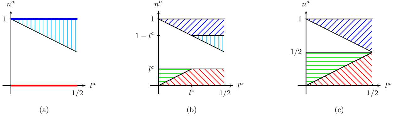
Fig. 3. Phase diagram for Situation 2: (a) l^c = 0 ; (b) l^c \in ]0, 1/2[ ; (c) l^c \rightarrow 1/2 . Color code: white=chaos, blue=cycle, cyan=fuzzy cycle, red=polarization, green=fuzzy polarization
