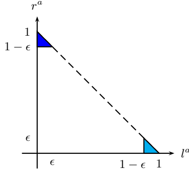
Fig. 5. Phase diagram for Situation 3, with l^c, r^c < \epsilon . Color code: blue=chaotic ‘no’ (13), cyan=chaotic ‘yes’ (14), white=chaos (20)
