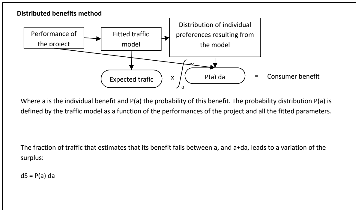
Figure 3: Distributed benefits method
