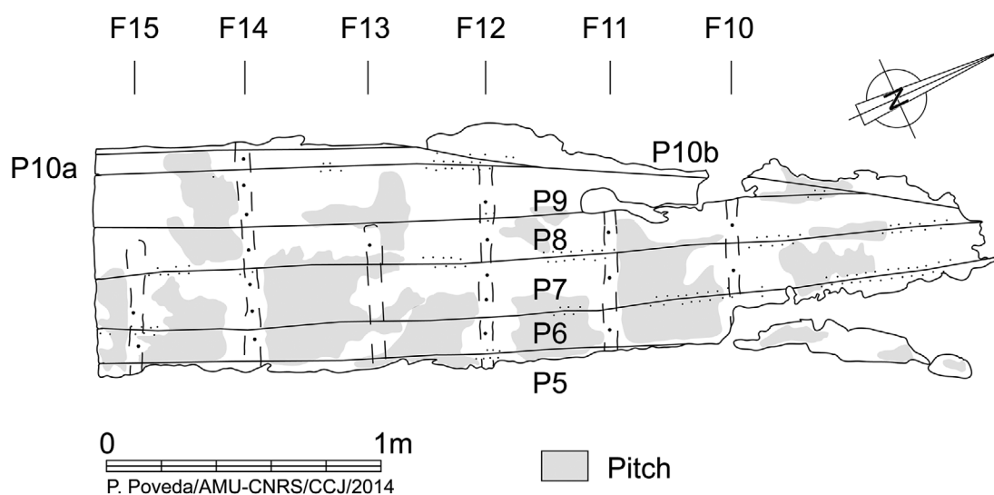
Figure 22. Caska 3: plan (drawing P. Poveda, AMU, CNRS, CCJ).
