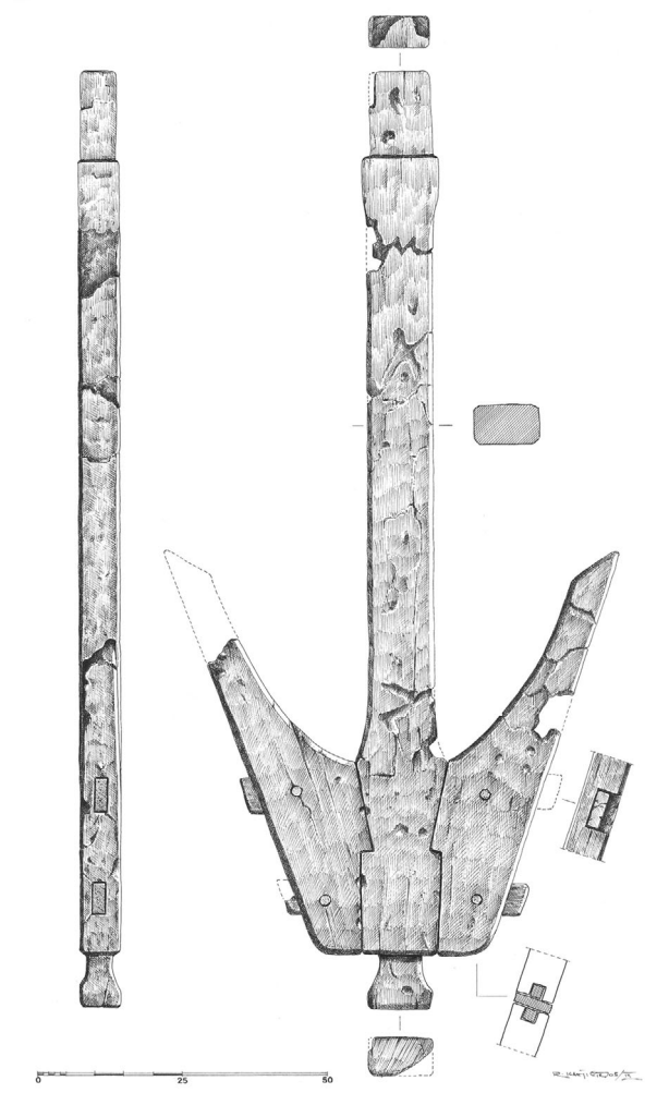
Figure 7. Wooden anchor found in 2005 (drawing K. Rončević, University of Zagreb).
