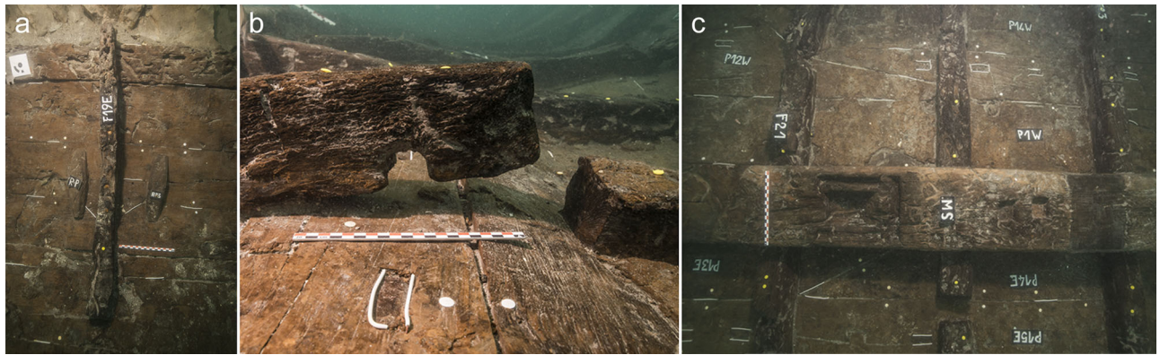
Figure 28. Caska 2: a) interior reinforcements on the port side; b) limber-hole on a half-frame. The white wire indicates the position of a patch-tenon on the garboard; c) mast step and the others recesses for stanchions on the keelson/mast-step (photos T. Seguin).
