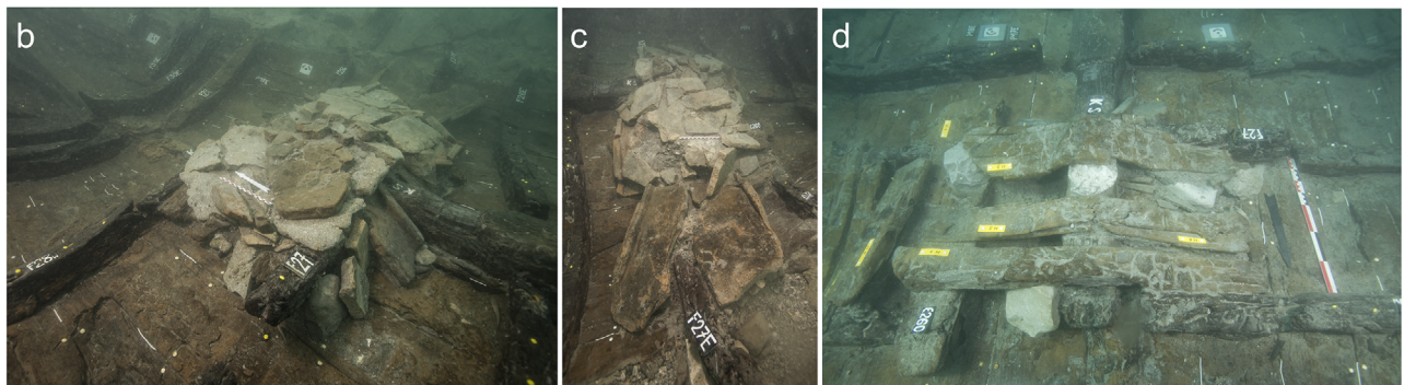
Figure 29. Caska 2: a) hearth (drawing P. Poveda, AMU, CNRS, CCJ); views of the hearth; b) from the South-West; c) from the East (photos T. Seguin); d) layer of planks supporting the hearth from the North (photo S. Govorčin, University of Zadar).
