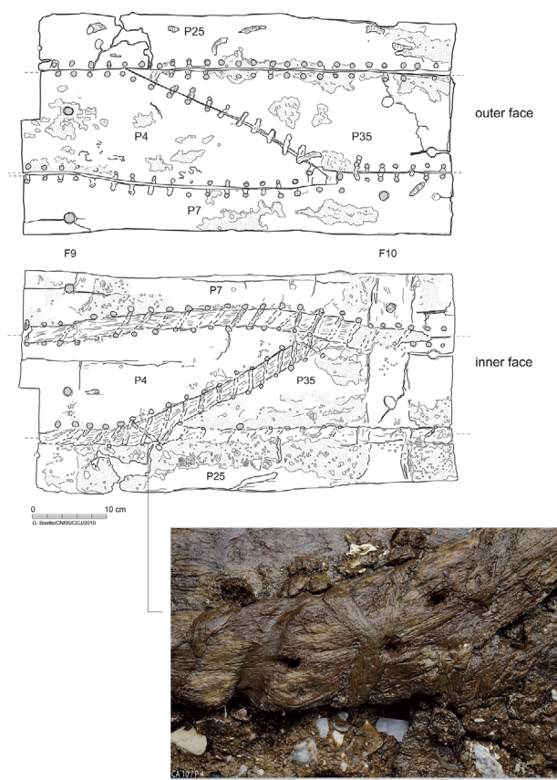
Figure 19. Caska 1: sewing pattern (drawings G. Boetto; photo L. Damelet, AMU, CNRS, CCJ).
