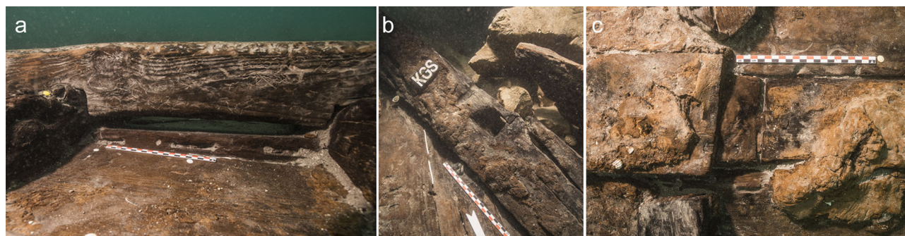
Figure 26. Caska 2: a) upper part of the keel without chamfer. The keelson/mast step is carved to accommodate on the frames and worked to allow the bilge water to circulate; b) recess on the upper surface of the stern transitional timber; c) scarf between the keel (right) and the stem transitional timber (left). Note the yellow pitch covering the hull (photos T. Seguin).
