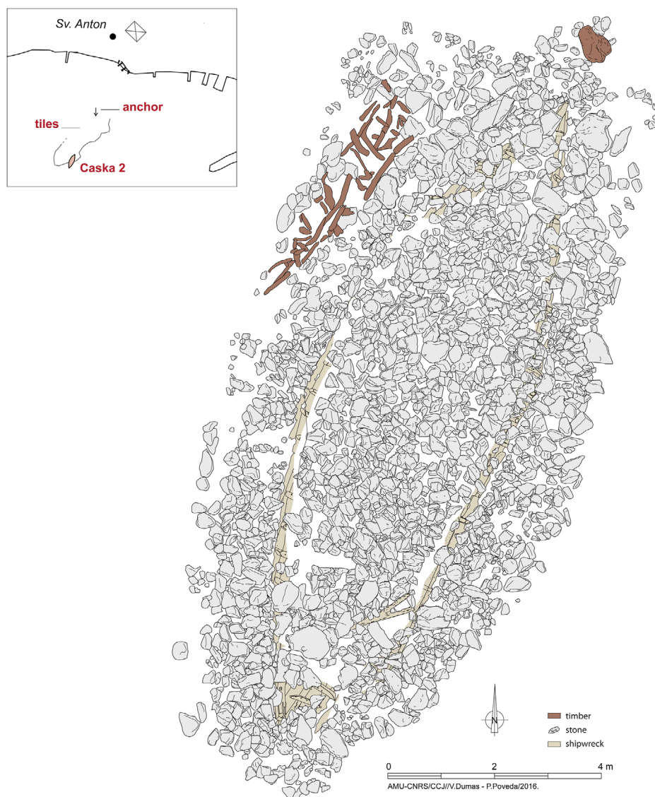
Figure 8. Zone D with the scuttled ship Caska 2 (drawing V. Dumas and P. Poveda, AMU, CNRS, CCJ).
