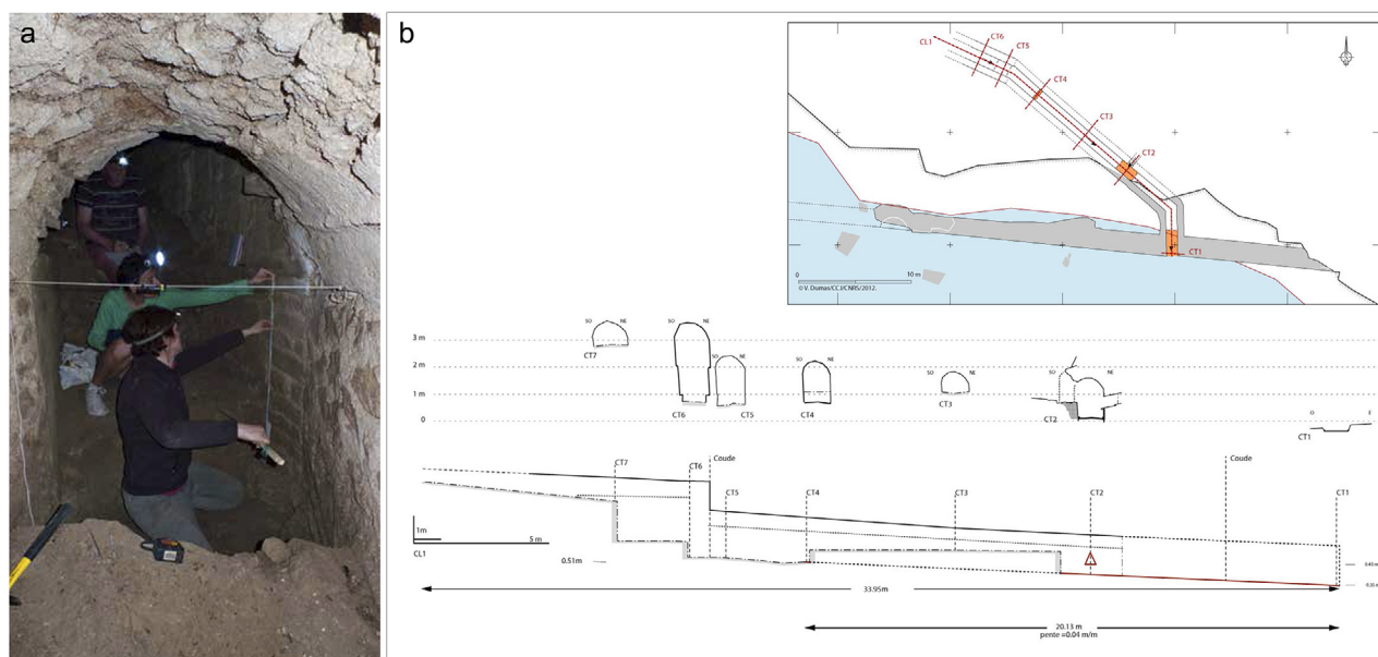
Figure 5. a) Measuring of the underground canal (photo Ph. Groscaux, AMU, CNRS, CCJ); b) plan and cross-section of the underground canal/tunnel (drawing V. Dumas, AMU, CNRS).
