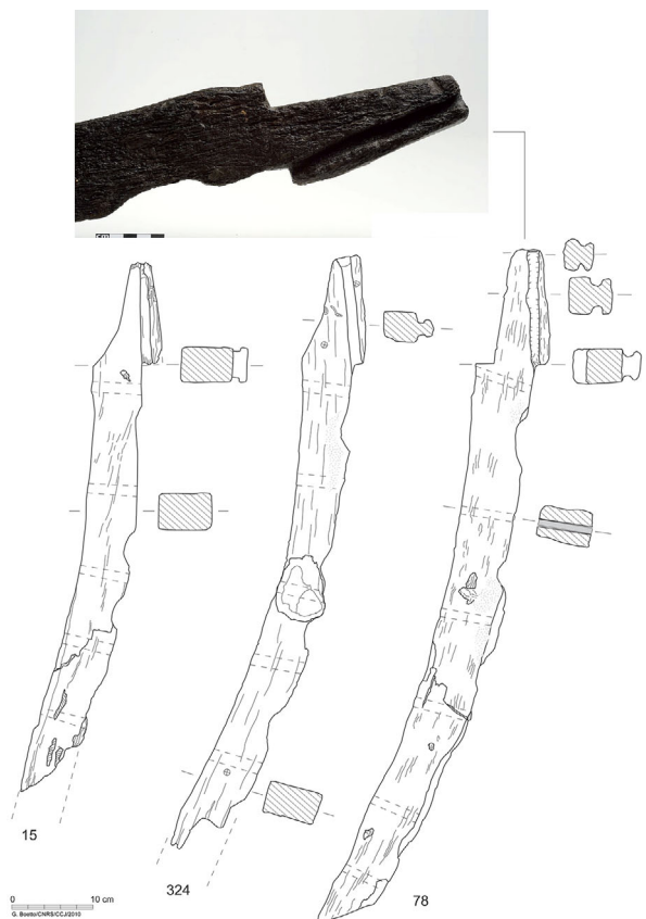
Figure 17. Caska 1: worked futtocks nos 15, 78 and 324 (drawings G. Boetto, photo L. Damelet, AMU, CNRS, CCJ).
