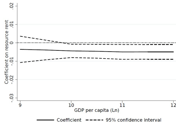
Figure 8: Recursive estimation on the coefficient of interest.
