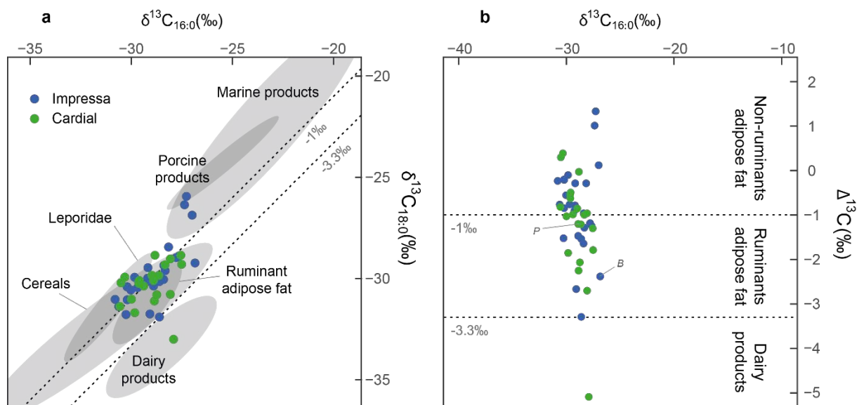
Figure 5: a) \delta^{13}C values of fatty acids ( C_{16:0} and C_{18:0} ) in pottery from the Pendimoun rock-shelter. Ellipses (95% confidence) are calculated from modern reference substances from the UK, Finland, Russia, Canada, Kazakhstan, Italy and Southern France (Cramp and Evershed, 2014; Debono Spiteri, 2012; Dudd, 1999; Outram et al., 2009; Pääkkönen et al., 2020; Taché and Craig, 2015; and this study). b) Plot of the \Delta^{13}C (difference between the \delta^{13}C values of the C_{16:0} and C_{18:0} fatty acids) and \delta^{13}C_{16:0} . B: beeswax; P: plant epicuticular wax.
