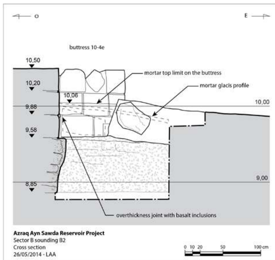
Fig.17: Cross section looking north of sounding B2 (LAA 2014).
