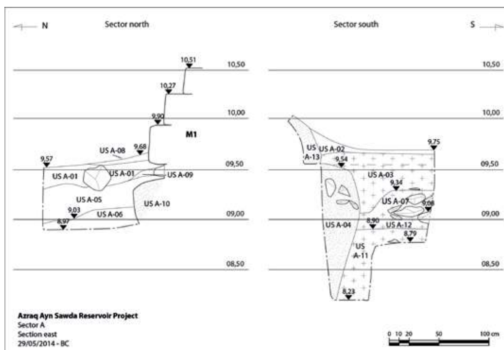
Fig.10a: Sections E of A south and A north (BC 2014).
