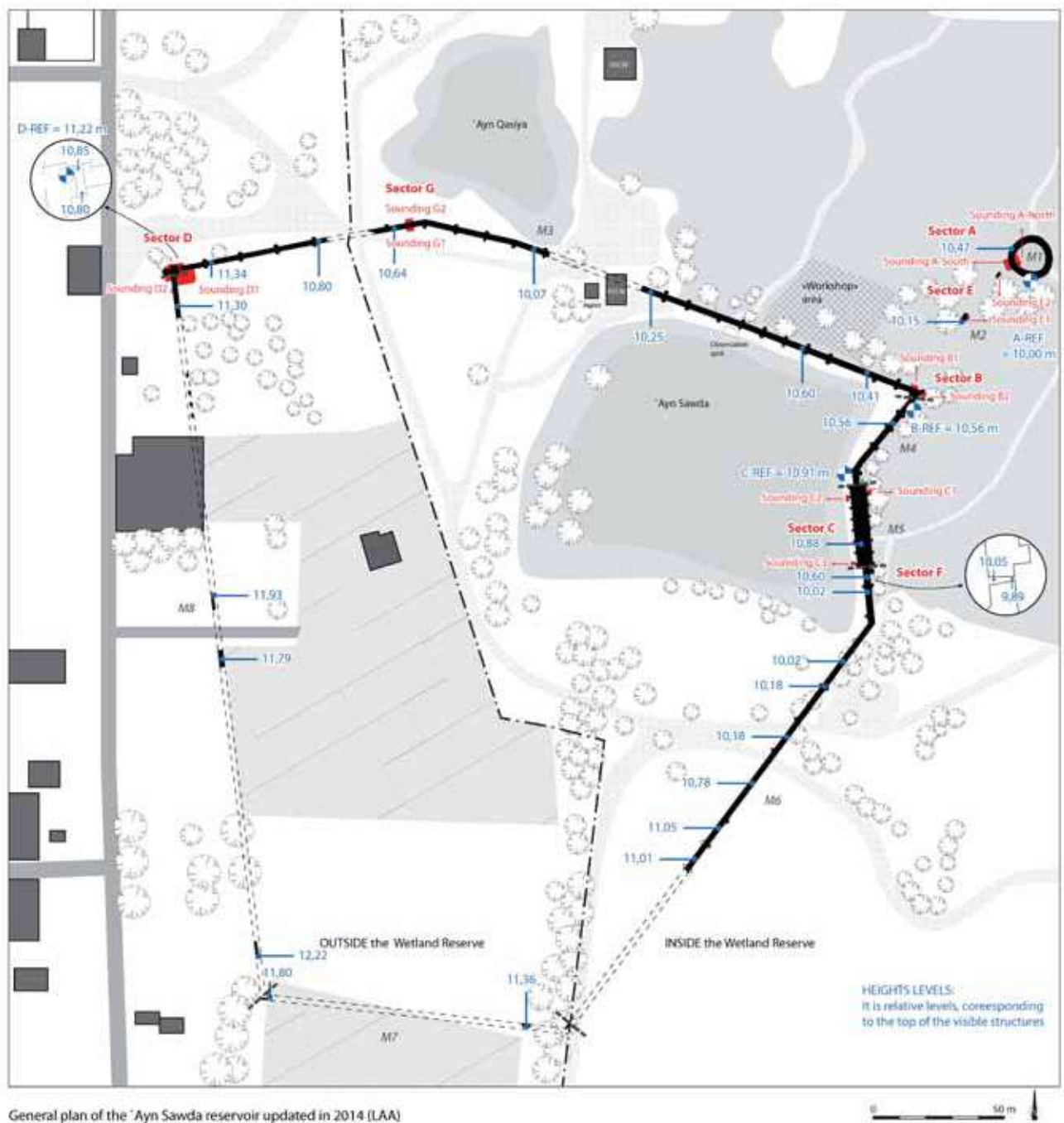
Fig.51: General plan of the reservoir with levels and sectors indications (LAA 2014).
