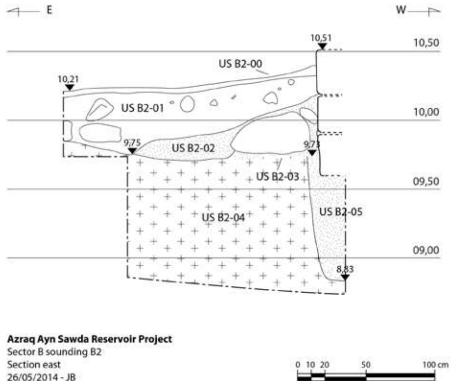
Fig.16: Section east of sounding B2 (JB 2014).
