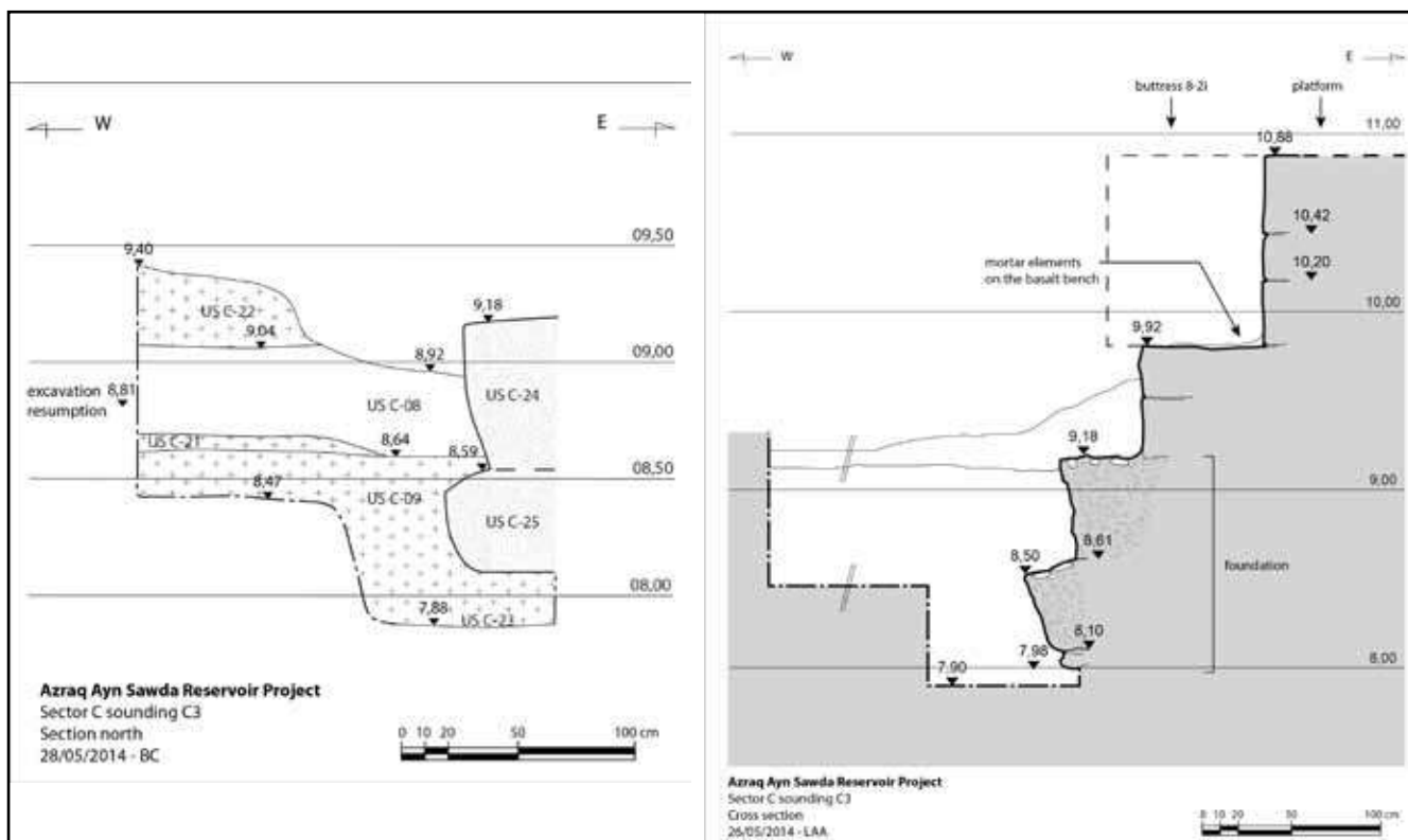
Fig.29: Section north of sounding C3 (BC and LAA 2014).
