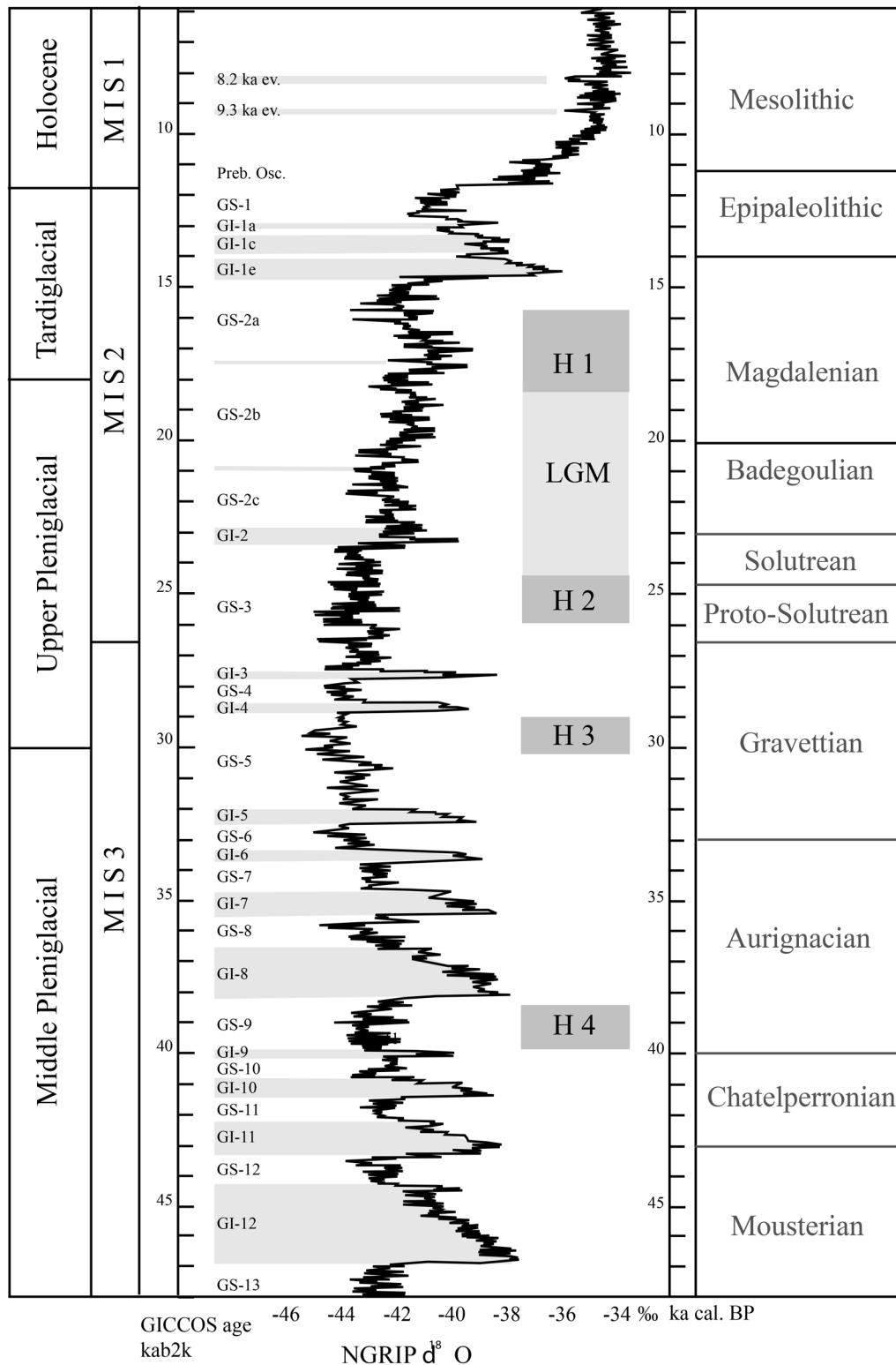
Figure 1. Chrono-climatic and chrono-cultural framework, after Aubry and Almeida (2013) and Blockley et al. (2012). Preb. Osc. : preboreal oscillations; GI : Greenland interstadial; GS : Greenland stadial; ev. : event.
