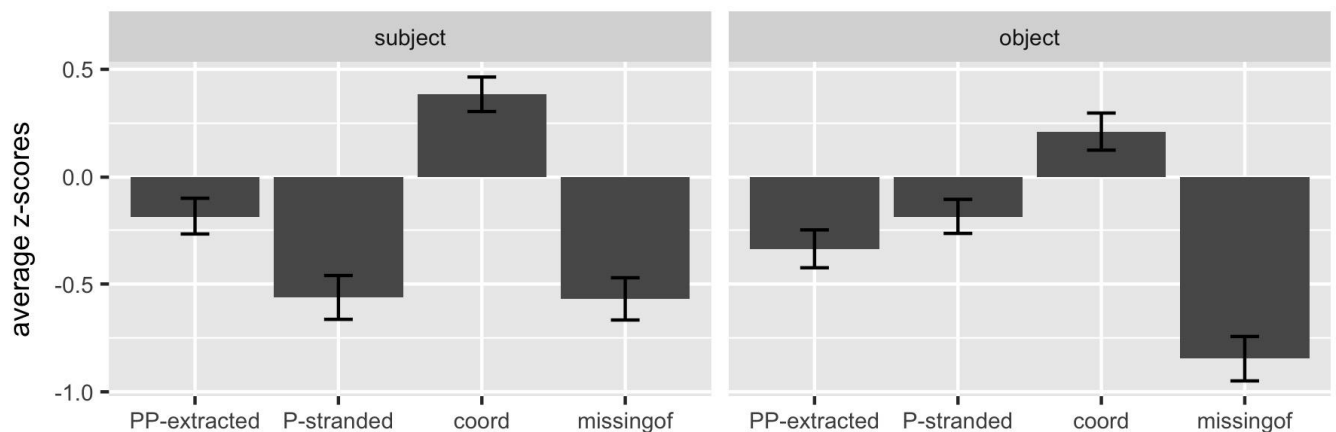
Figure 2: Condition means and 95% confidence intervals for z-scores of all conditions Experiment 2, based on the standard error of the condition mean as estimated by the regression.
