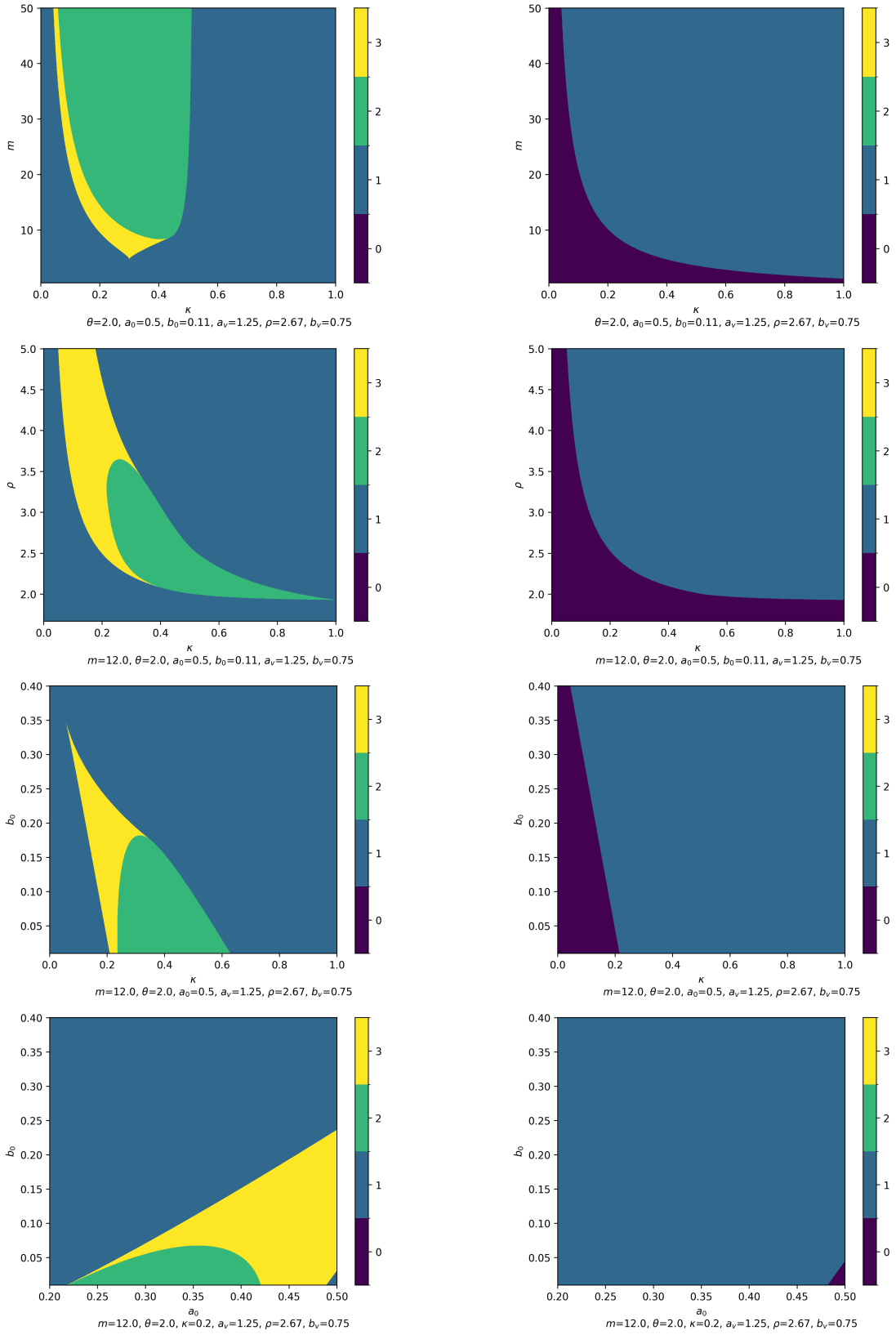
(a) Number of equilibria
