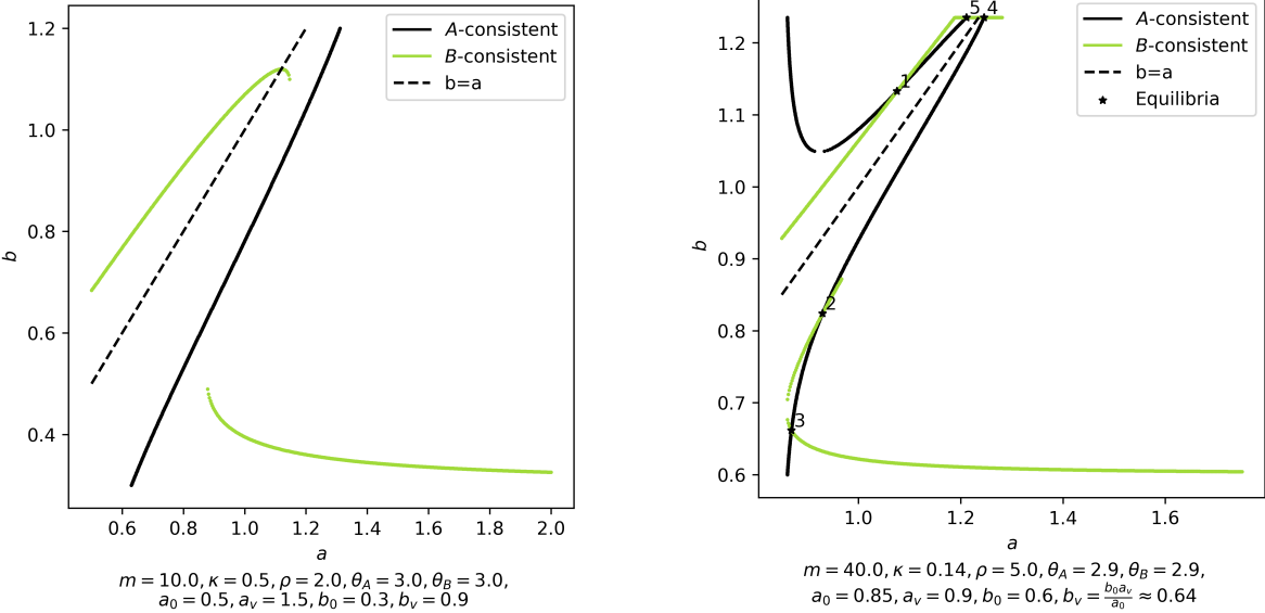
(a) An example of failure of equilibrium existence
