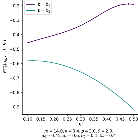
Figure 8: Utility from deviating from each equilibrium candidate
