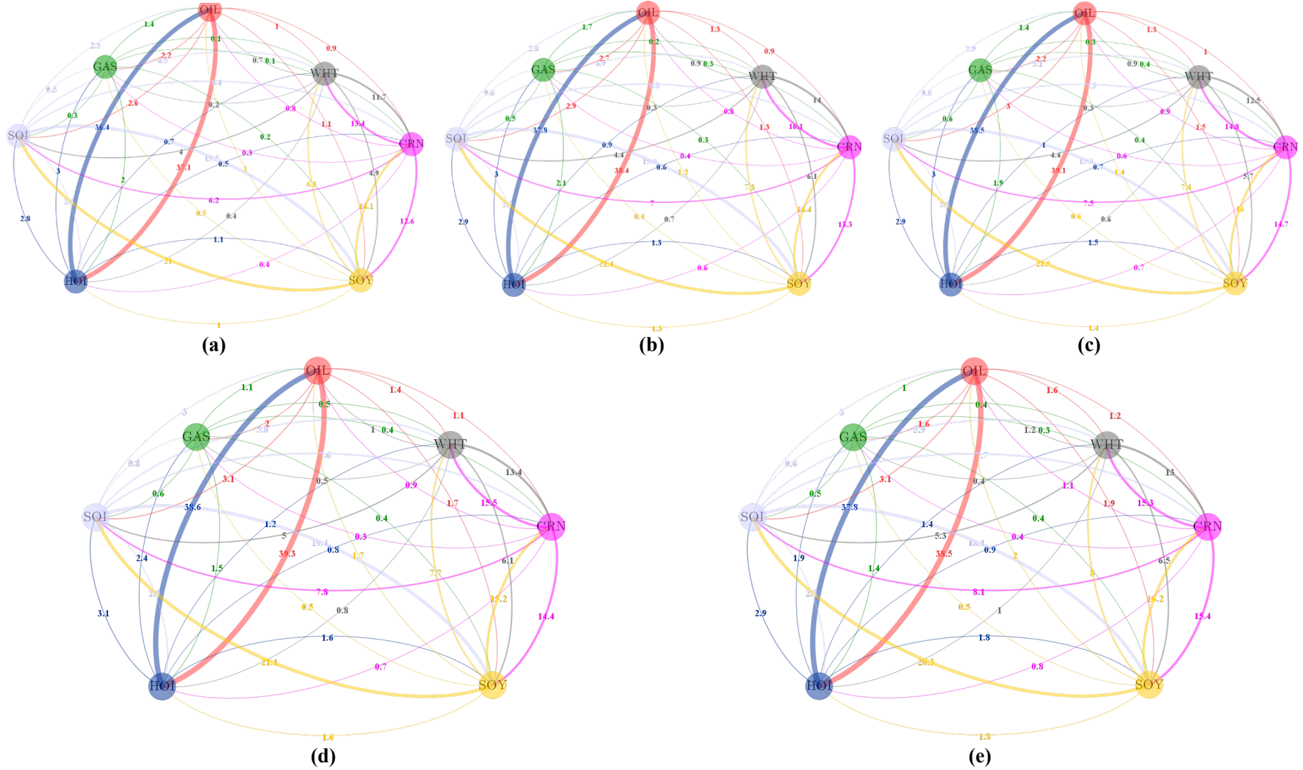
Fig. 3 Directional Spillovers network graph – Basket 2 [Full sample estimations]
