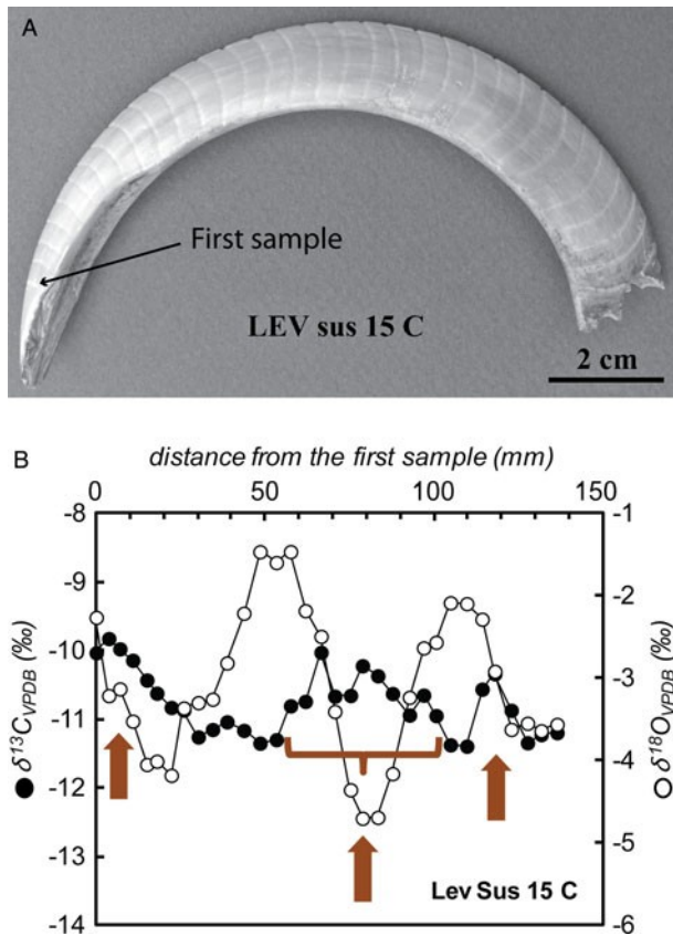
Figure 6. Intra-tooth \delta^{18}O (open circles) and \delta^{13}C (filled circles) variations (B) measured in a male lower canine (A) dated to the early second century BC from Levroux Les Arènes. The arrows indicate the seasonal increase in \delta^{13}C values, a pattern suggesting the seasonal consumption of forest fruits in autumn and winter.
