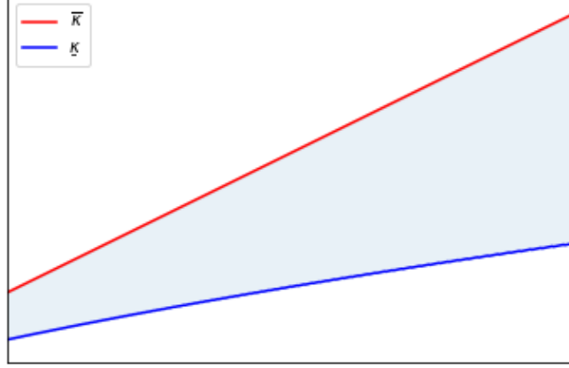
Figure 3. Wealth utility factors \kappa that ensure multiplicity when varies the private consumption externality \vartheta on the government's utility
