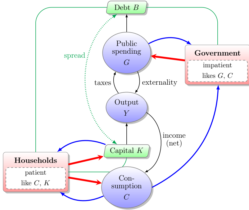
Figure 1. A model with two utility-optimizing agents
