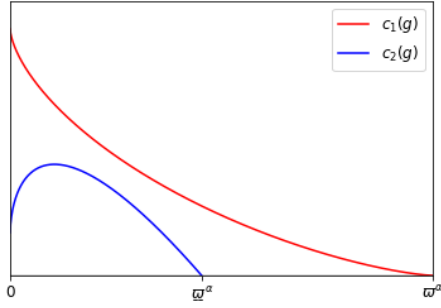
(a) c_1 above c_2
