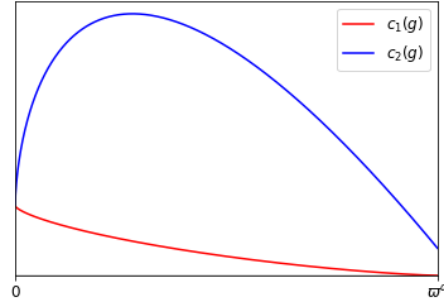
(b) c_2 above c_1
