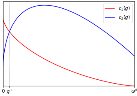
(c) Unique steady state with c'_2(g^*) > c'_1(g^*)
