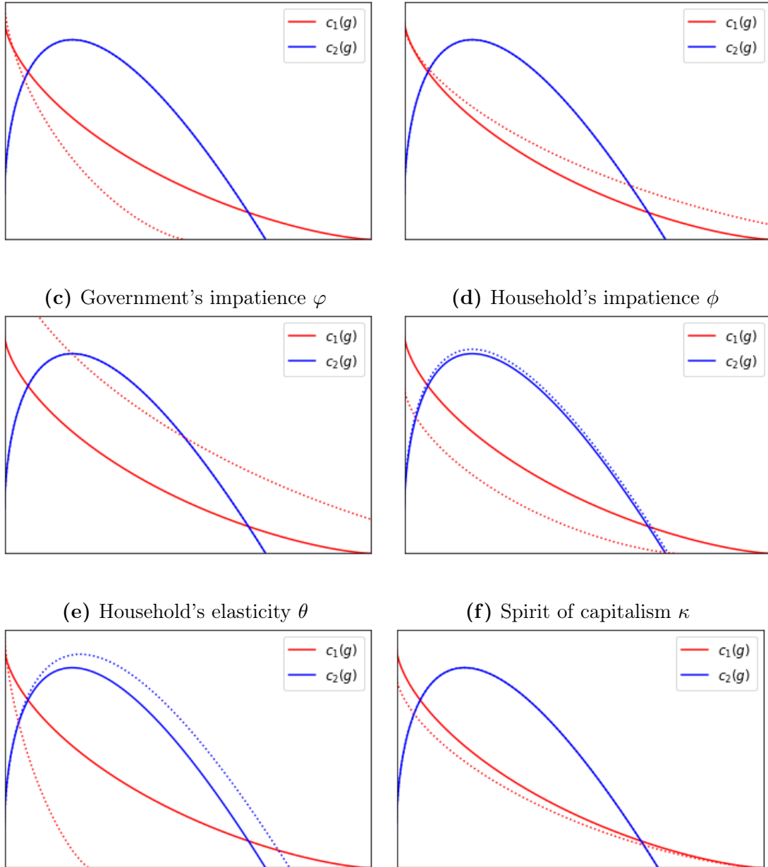
Figure E.1. Parameter sensitivity of the two characteristic functions (a) Consumption externality \vartheta (b) Government's elasticity \varsigma
