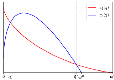
(e) Dual steady states
